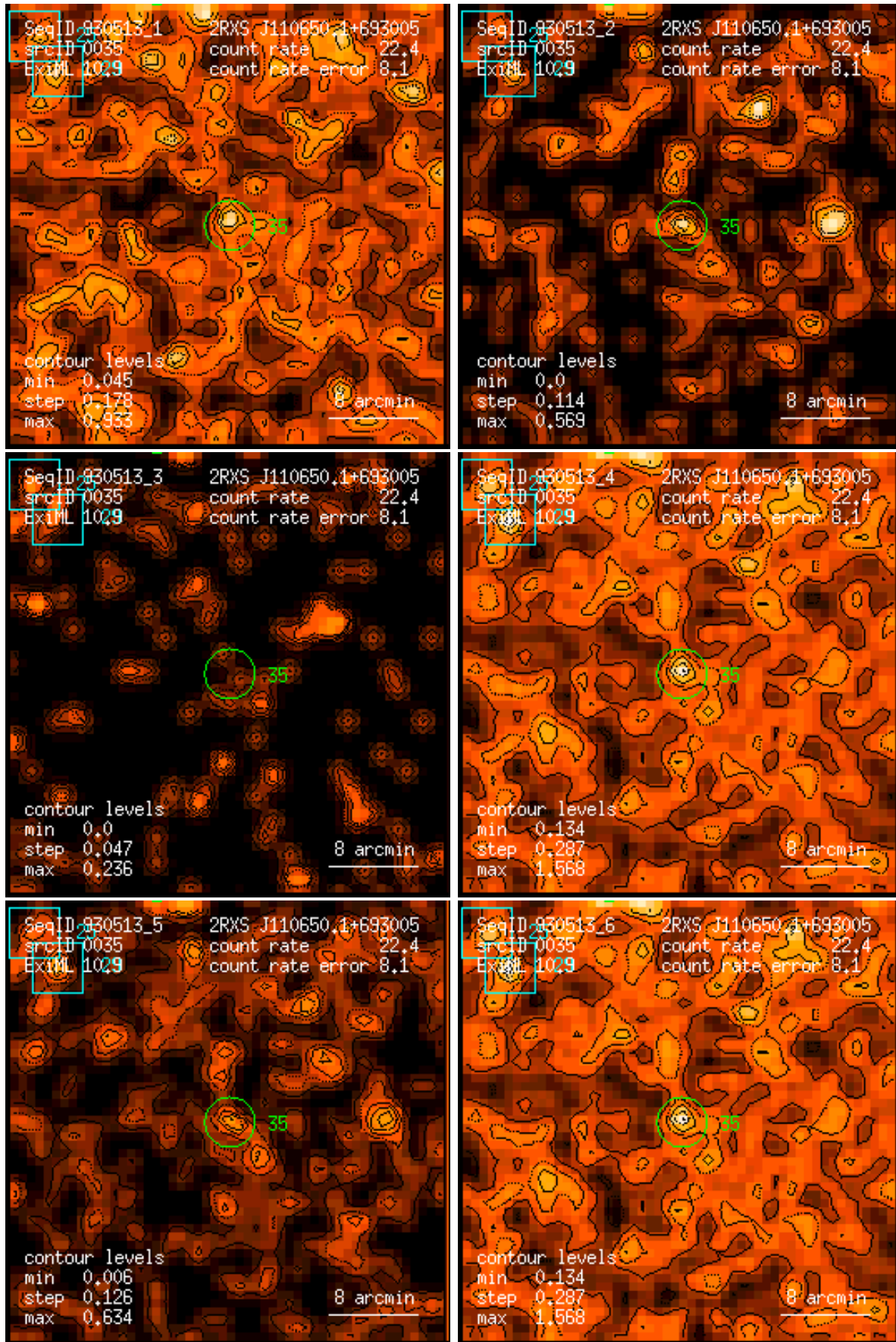
Figure 35: RASS 930513: detection 0035: band rate images, Gaussian filter: (1) PSPC channels 11 – 41, (2) 52 – 90, (3) 91 – 201, (4) 11 – 235, (5) 52 – 201, (6) 11 – 201. Broad band rates in counts/ks. Band rate contour levels in counts/ks/arcmin 2 .
