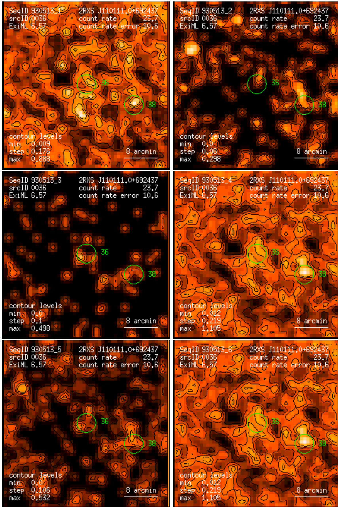
Figure 36: RASS 930513: detection 0036: band rate images, Gaussian filter: (1) PSPC channels 11 – 41, (2) 52 – 90, (3) 91 – 201, (4) 11 – 235, (5) 52 – 201, (6) 11 – 201. Broad band rates in counts/ks. Band rate contour levels in counts/ks/arcmin 2 .
