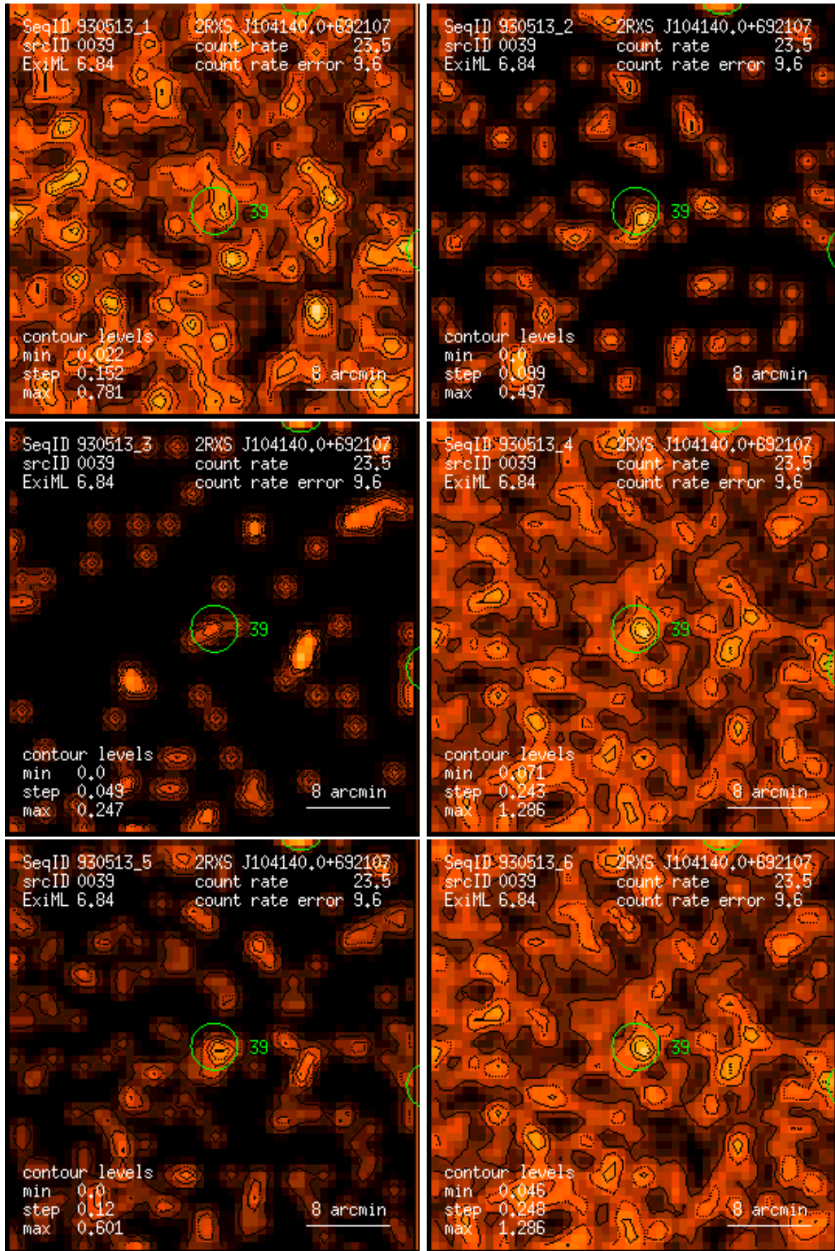
Figure 39: RASS 930513: detection 0039: band rate images, Gaussian filter: (1) PSPC channels 11 – 41, (2) 52 – 90, (3) 91 – 201, (4) 11 – 235, (5) 52 – 201, (6) 11 – 201. Broad band rates in counts/ks. Band rate contour levels in counts/ks/arcmin 2 .
