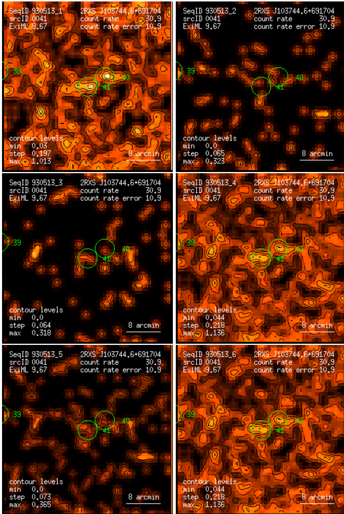
Figure 41: RASS 930513: detection 0041: band rate images, Gaussian filter: (1) PSPC channels 11 – 41, (2) 52 – 90, (3) 91 – 201, (4) 11 – 235, (5) 52 – 201, (6) 11 – 201. Broad band rates in counts/ks. Band rate contour levels in counts/ks/arcmin 2 .
