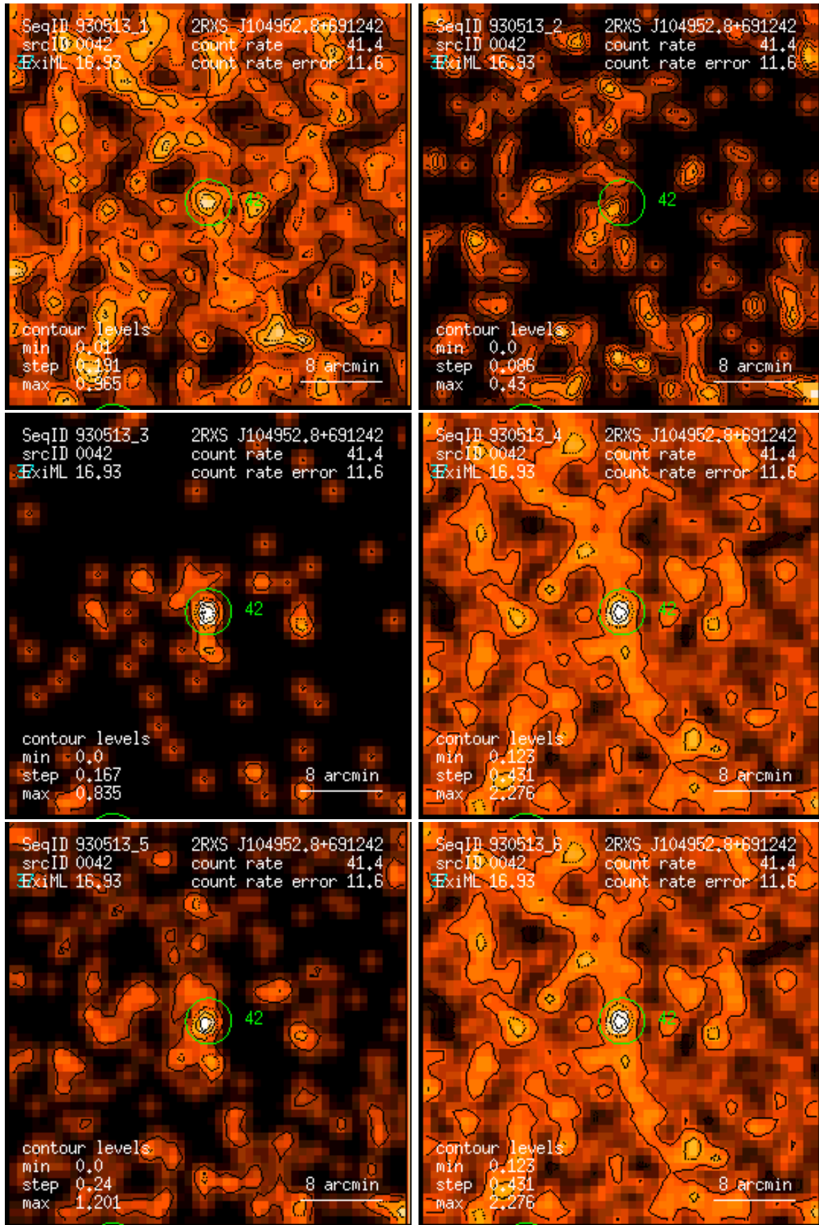
Figure 42: RASS 930513: detection 0042: band rate images, Gaussian filter: (1) PSPC channels 11 – 41, (2) 52 – 90, (3) 91 – 201, (4) 11 – 235, (5) 52 – 201, (6) 11 – 201. Broad band rates in counts/ks. Band rate contour levels in counts/ks/arcmin 2 .
