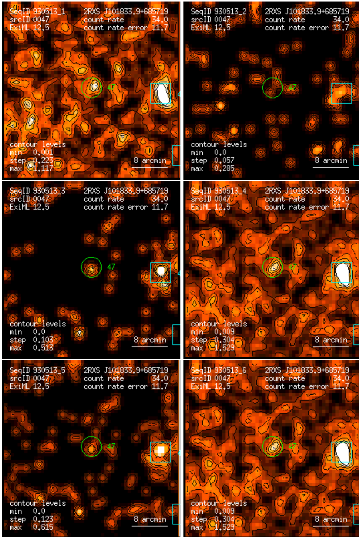
Figure 47: RASS 930513: detection 0047: band rate images, Gaussian filter: (1) PSPC channels 11 – 41, (2) 52 – 90, (3) 91 – 201, (4) 11 – 235, (5) 52 – 201, (6) 11 – 201. Broad band rates in counts/ks. Band rate contour levels in counts/ks/arcmin 2 .
