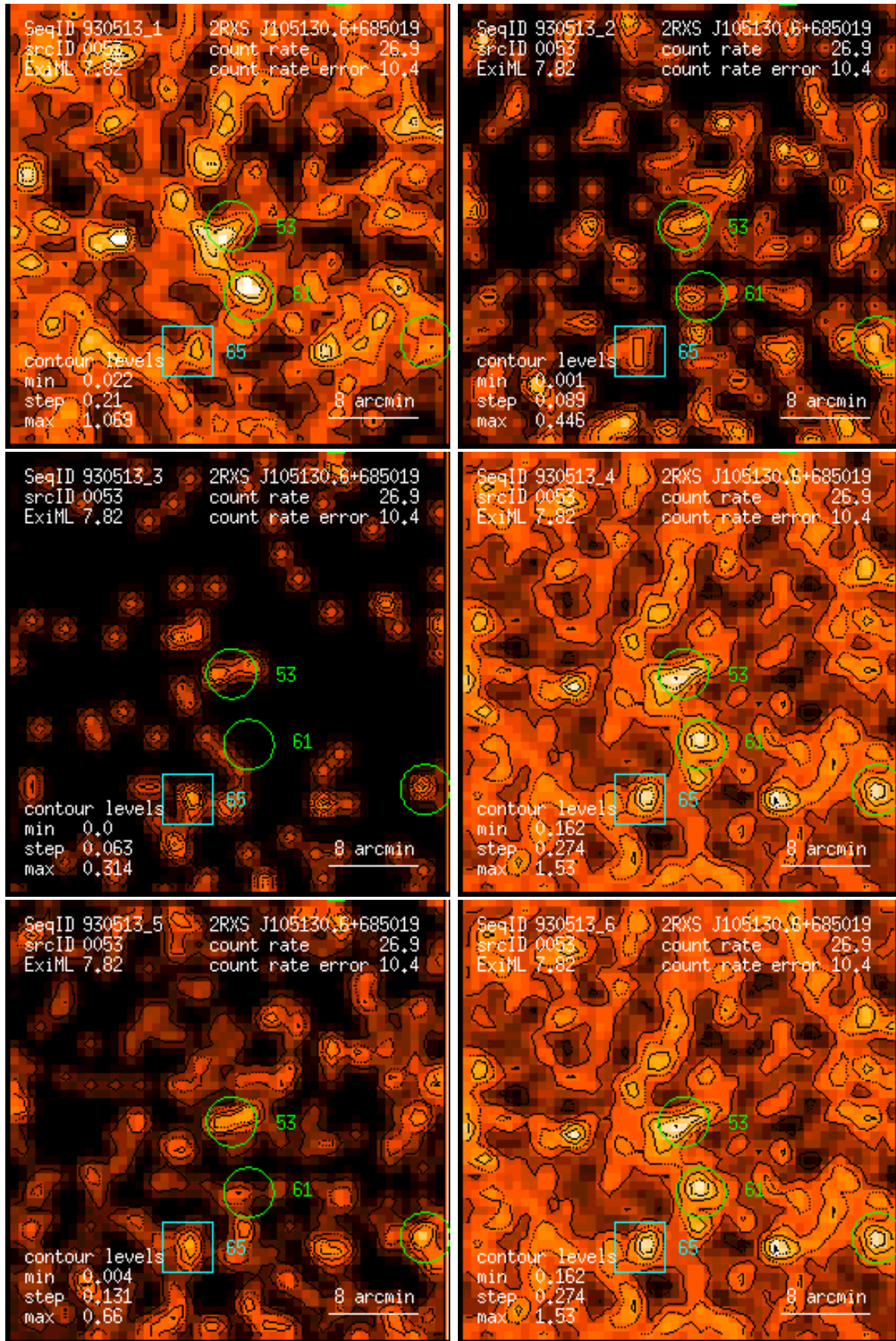
Figure 53: RASS 930513: detection 0053: band rate images, Gaussian filter: (1) PSPC channels 11 – 41, (2) 52 – 90, (3) 91 – 201, (4) 11 – 235, (5) 52 – 201, (6) 11 – 201. Broad band rates in counts/ks. Band rate contour levels in counts/ks/arcmin 2 .
