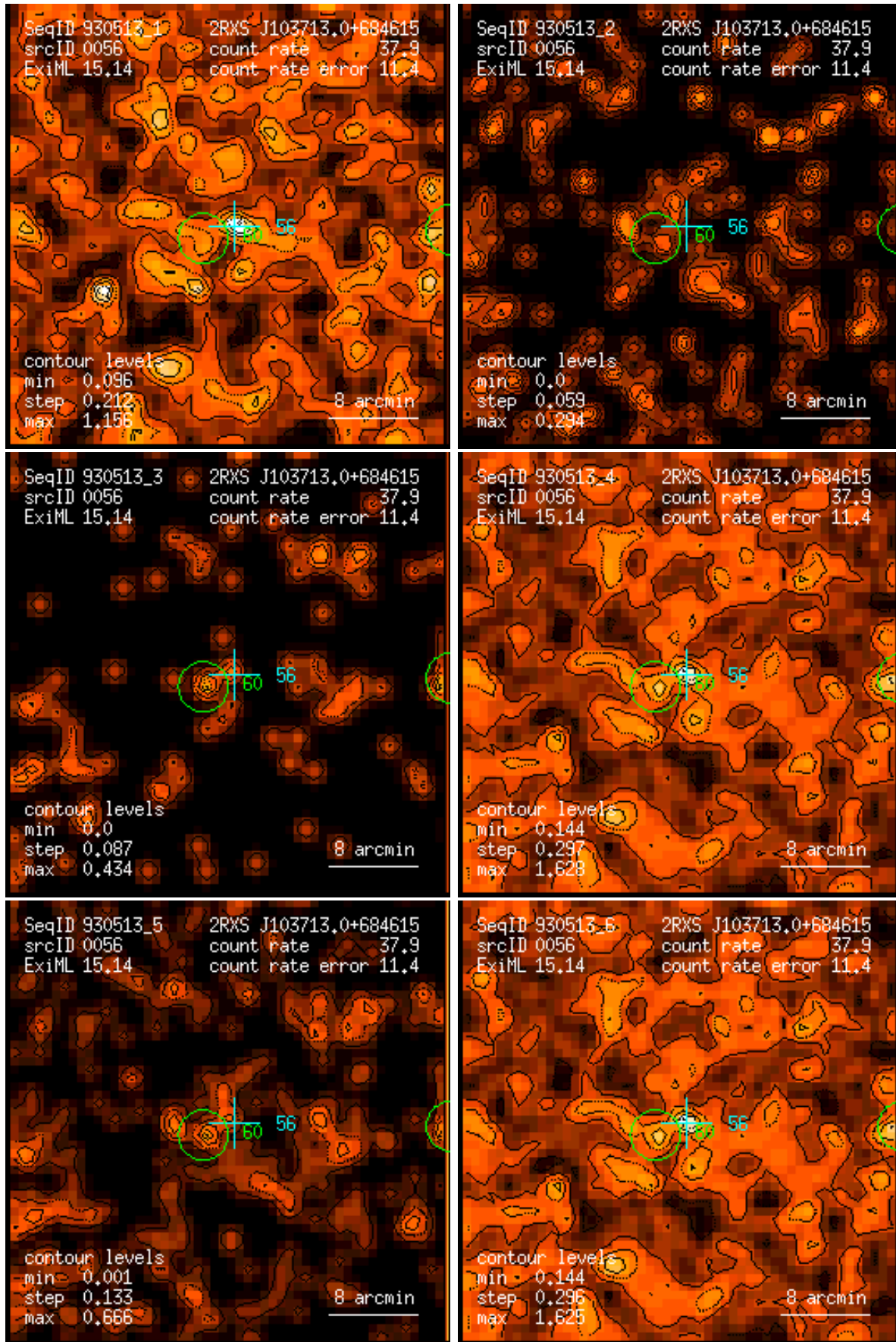
Figure 56: RASS 930513: detection 0056: band rate images, Gaussian filter: (1) PSPC channels 11 – 41, (2) 52 – 90, (3) 91 – 201, (4) 11 – 235, (5) 52 – 201, (6) 11 – 201. Broad band rates in counts/ks. Band rate contour levels in counts/ks/arcmin 2 .
