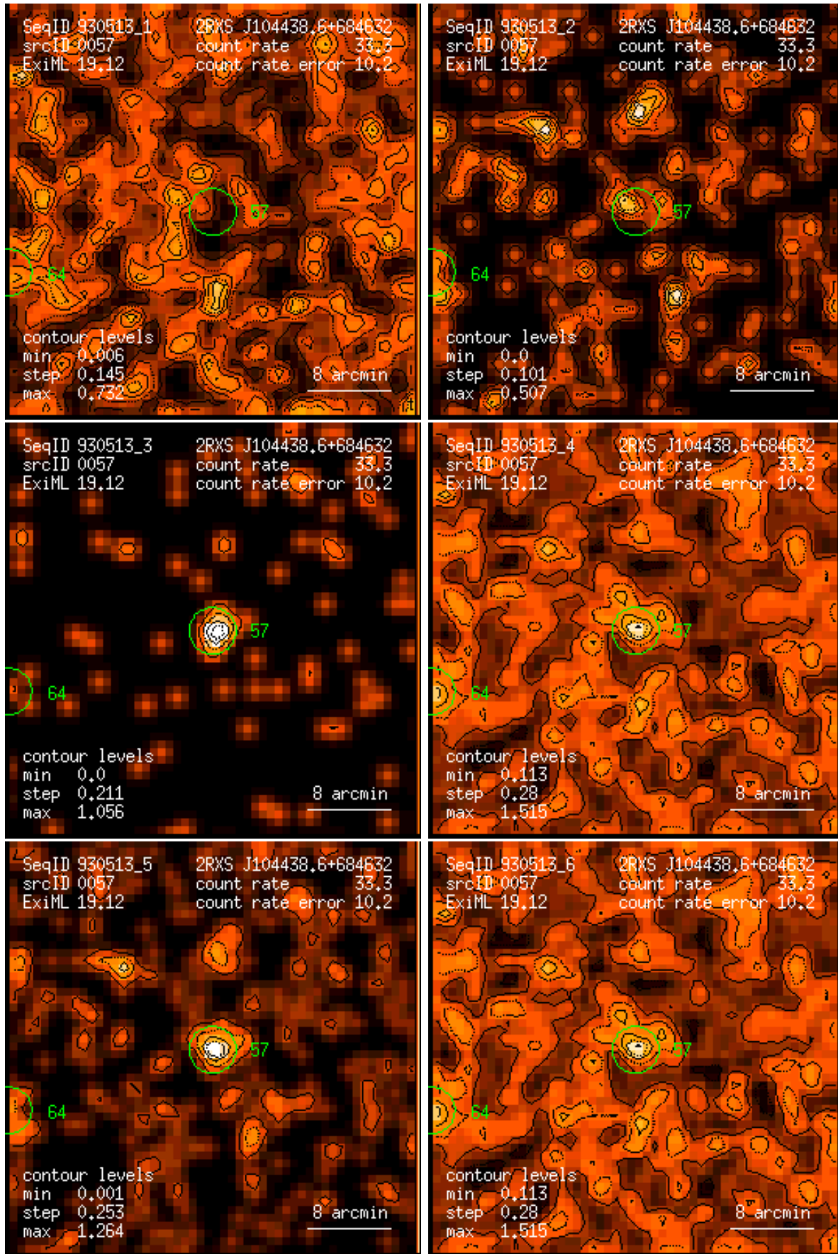
Figure 57: RASS 930513: detection 0057: band rate images, Gaussian filter: (1) PSPC channels 11 – 41, (2) 52 – 90, (3) 91 – 201, (4) 11 – 235, (5) 52 – 201, (6) 11 – 201. Broad band rates in counts/ks. Band rate contour levels in counts/ks/arcmin 2 .
