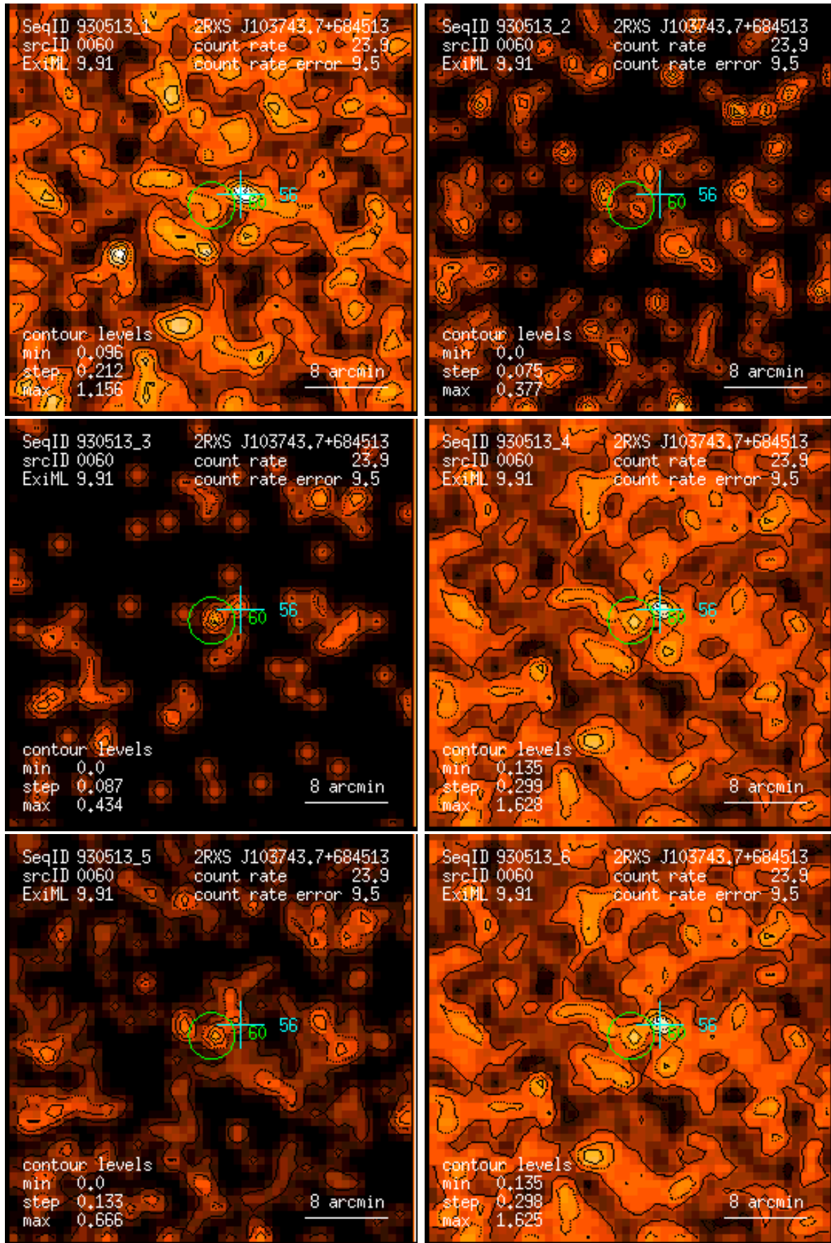
Figure 60: RASS 930513: detection 0060: band rate images, Gaussian filter: (1) PSPC channels 11 – 41, (2) 52 – 90, (3) 91 – 201, (4) 11 – 235, (5) 52 – 201, (6) 11 – 201. Broad band rates in counts/ks. Band rate contour levels in counts/ks/arcmin 2 .
