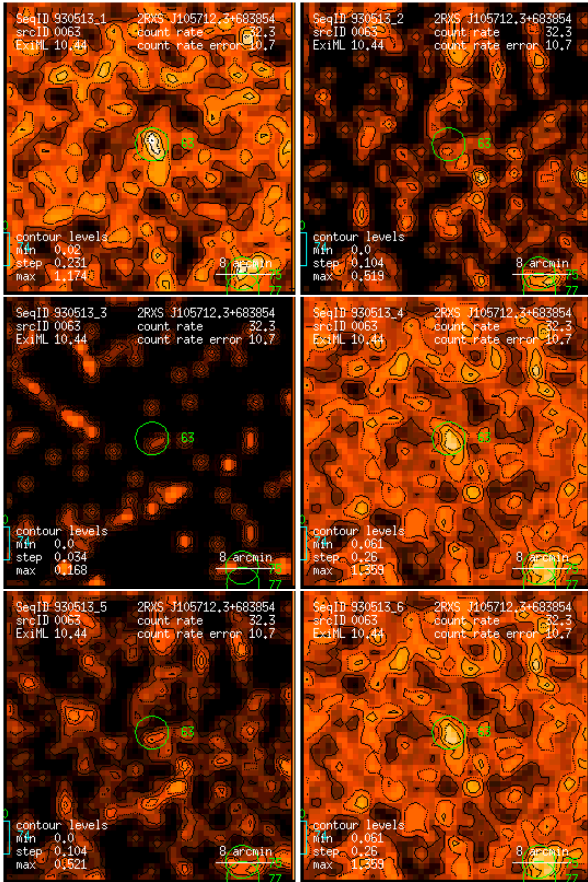
Figure 63: RASS 930513: detection 0063: band rate images, Gaussian filter: (1) PSPC channels 11 – 41, (2) 52 – 90, (3) 91 – 201, (4) 11 – 235, (5) 52 – 201, (6) 11 – 201. Broad band rates in counts/ks. Band rate contour levels in counts/ks/arcmin 2 .
