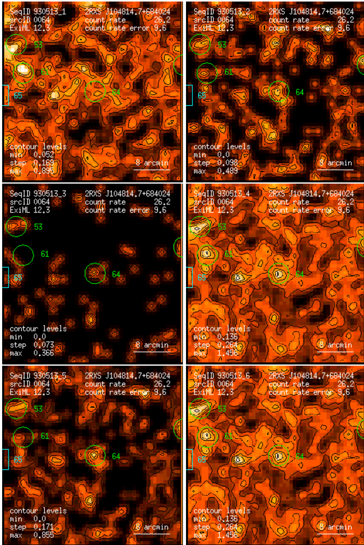
Figure 64: RASS 930513: detection 0064: band rate images, Gaussian filter: (1) PSPC channels 11 – 41, (2) 52 – 90, (3) 91 – 201, (4) 11 – 235, (5) 52 – 201, (6) 11 – 201. Broad band rates in counts/ks. Band rate contour levels in counts/ks/arcmin 2 .
