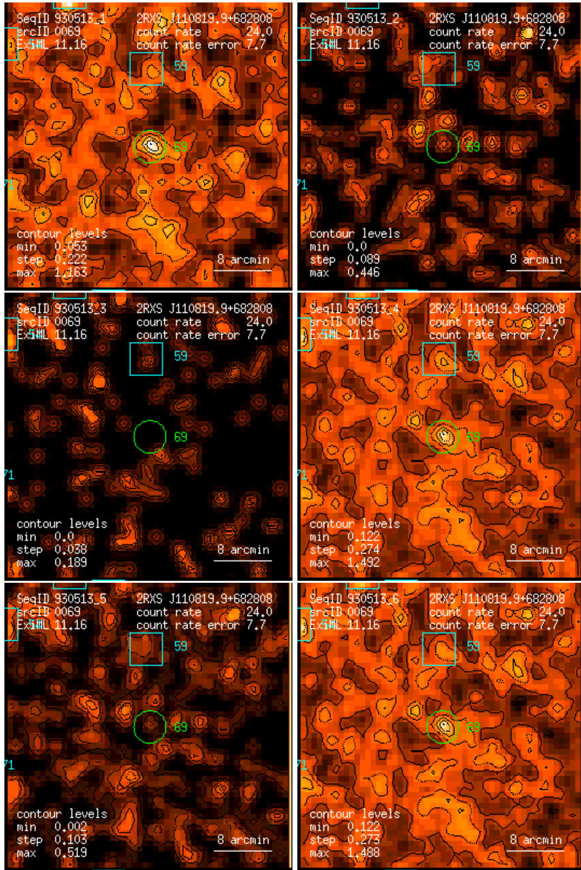
Figure 69: RASS 930513: detection 0069: band rate images, Gaussian filter: (1) PSPC channels 11 – 41, (2) 52 – 90, (3) 91 – 201, (4) 11 – 235, (5) 52 – 201, (6) 11 – 201. Broad band rates in counts/ks. Band rate contour levels in counts/ks/arcmin 2 .
