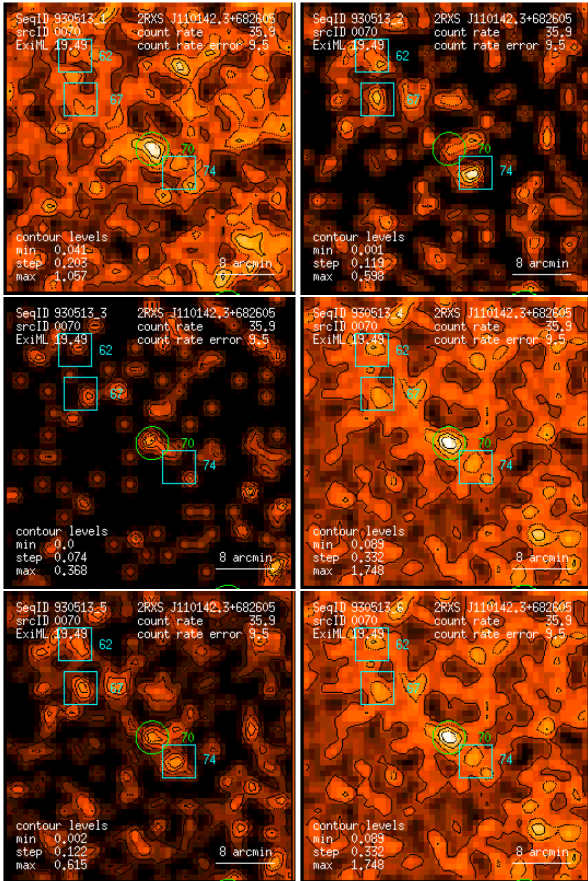
Figure 70: RASS 930513: detection 0070: band rate images, Gaussian filter: (1) PSPC channels 11 – 41, (2) 52 – 90, (3) 91 – 201, (4) 11 – 235, (5) 52 – 201, (6) 11 – 201. Broad band rates in counts/ks. Band rate contour levels in counts/ks/arcmin 2 .
