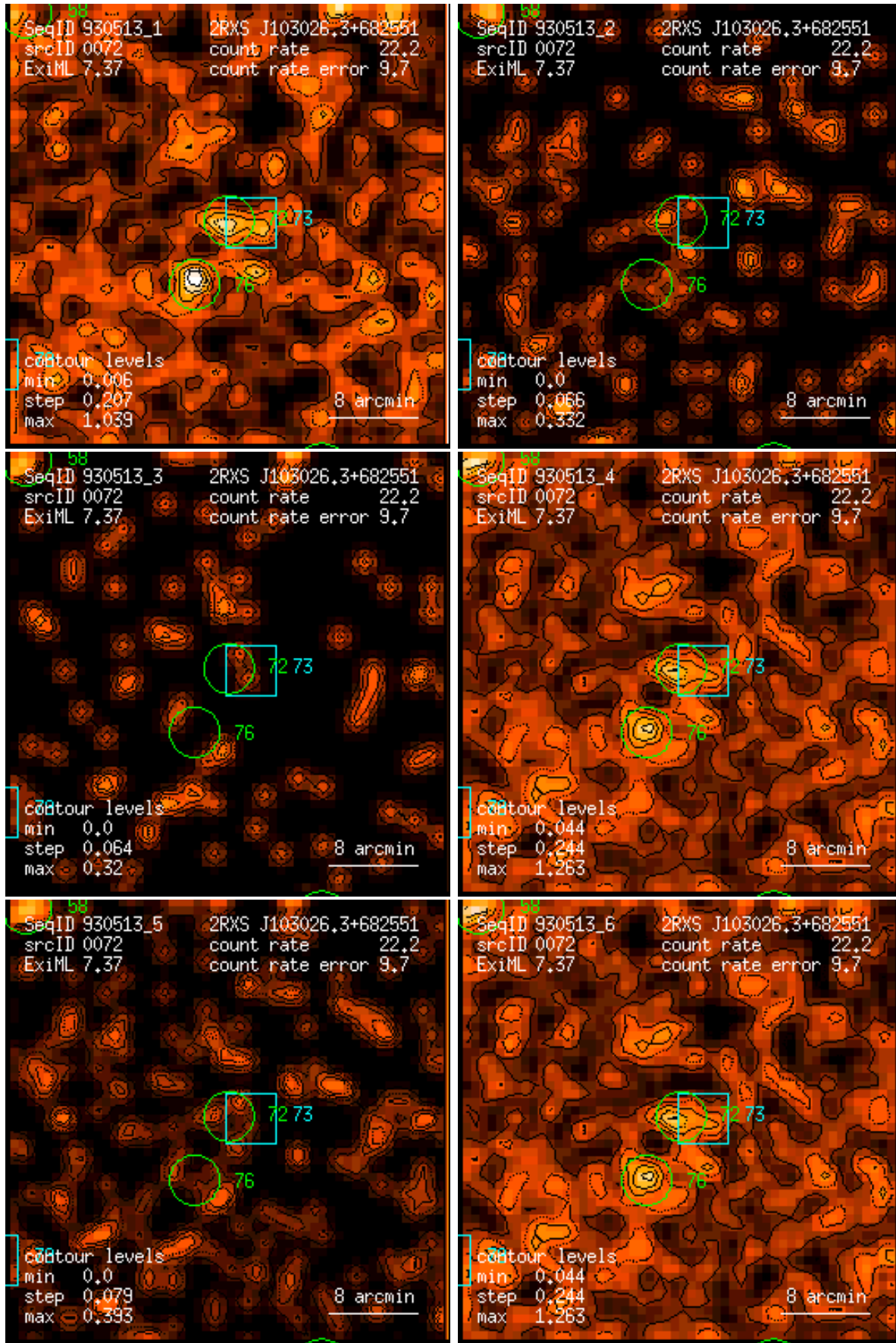
Figure 72: RASS 930513: detection 0072: band rate images, Gaussian filter: (1) PSPC channels 11 – 41, (2) 52 – 90, (3) 91 – 201, (4) 11 – 235, (5) 52 – 201, (6) 11 – 201. Broad band rates in counts/ks. Band rate contour levels in counts/ks/arcmin 2 .
