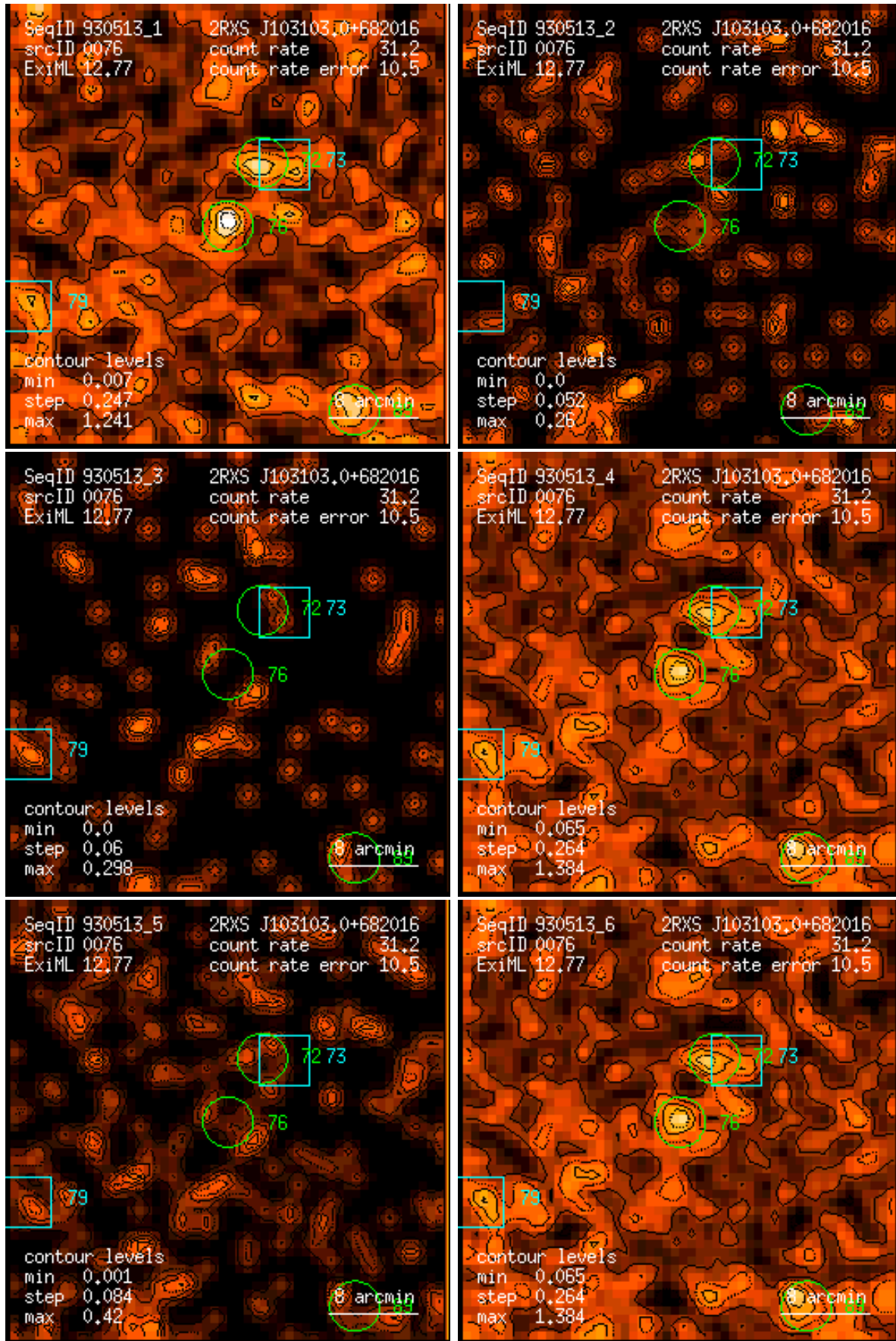
Figure 76: RASS 930513: detection 0076: band rate images, Gaussian filter: (1) PSPC channels 11 – 41, (2) 52 – 90, (3) 91 – 201, (4) 11 – 235, (5) 52 – 201, (6) 11 – 201. Broad band rates in counts/ks. Band rate contour levels in counts/ks/arcmin 2 .
