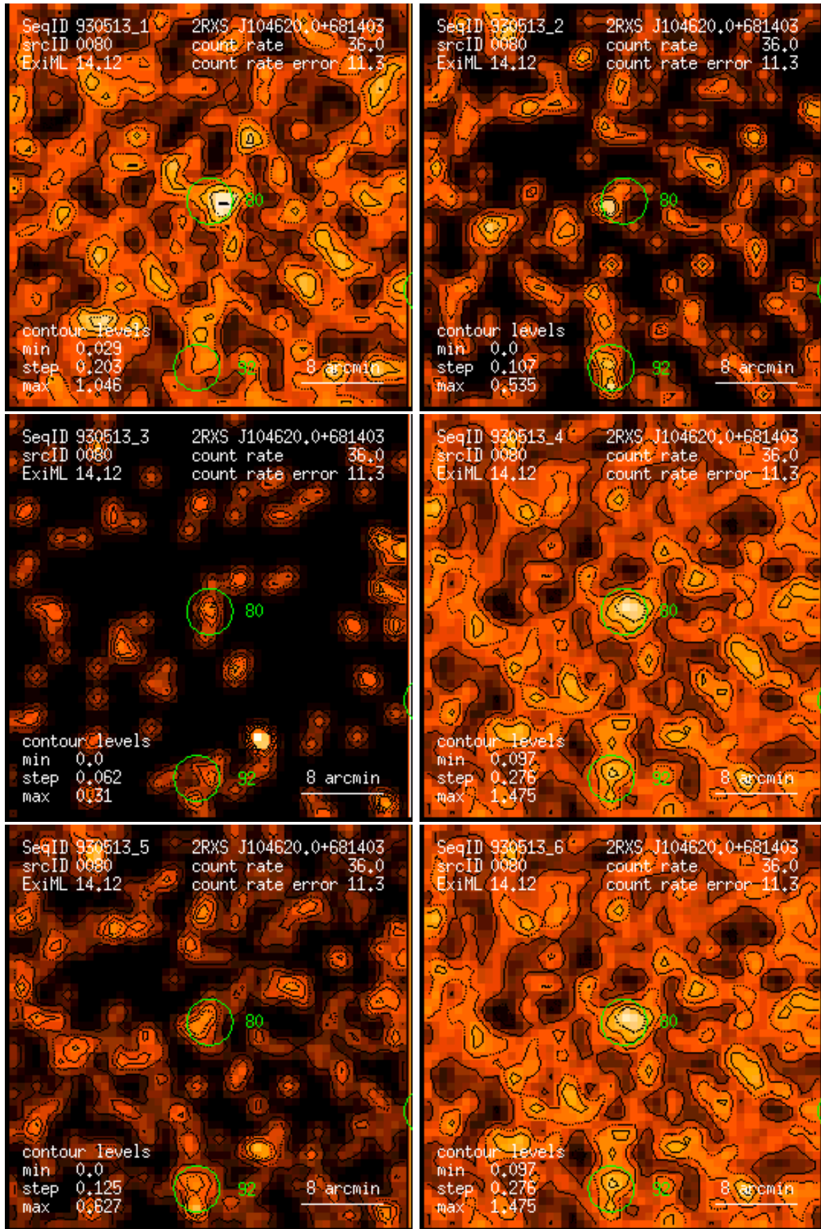
Figure 80: RASS 930513: detection 0080: band rate images, Gaussian filter: (1) PSPC channels 11 – 41, (2) 52 – 90, (3) 91 – 201, (4) 11 – 235, (5) 52 – 201, (6) 11 – 201. Broad band rates in counts/ks. Band rate contour levels in counts/ks/arcmin 2 .
