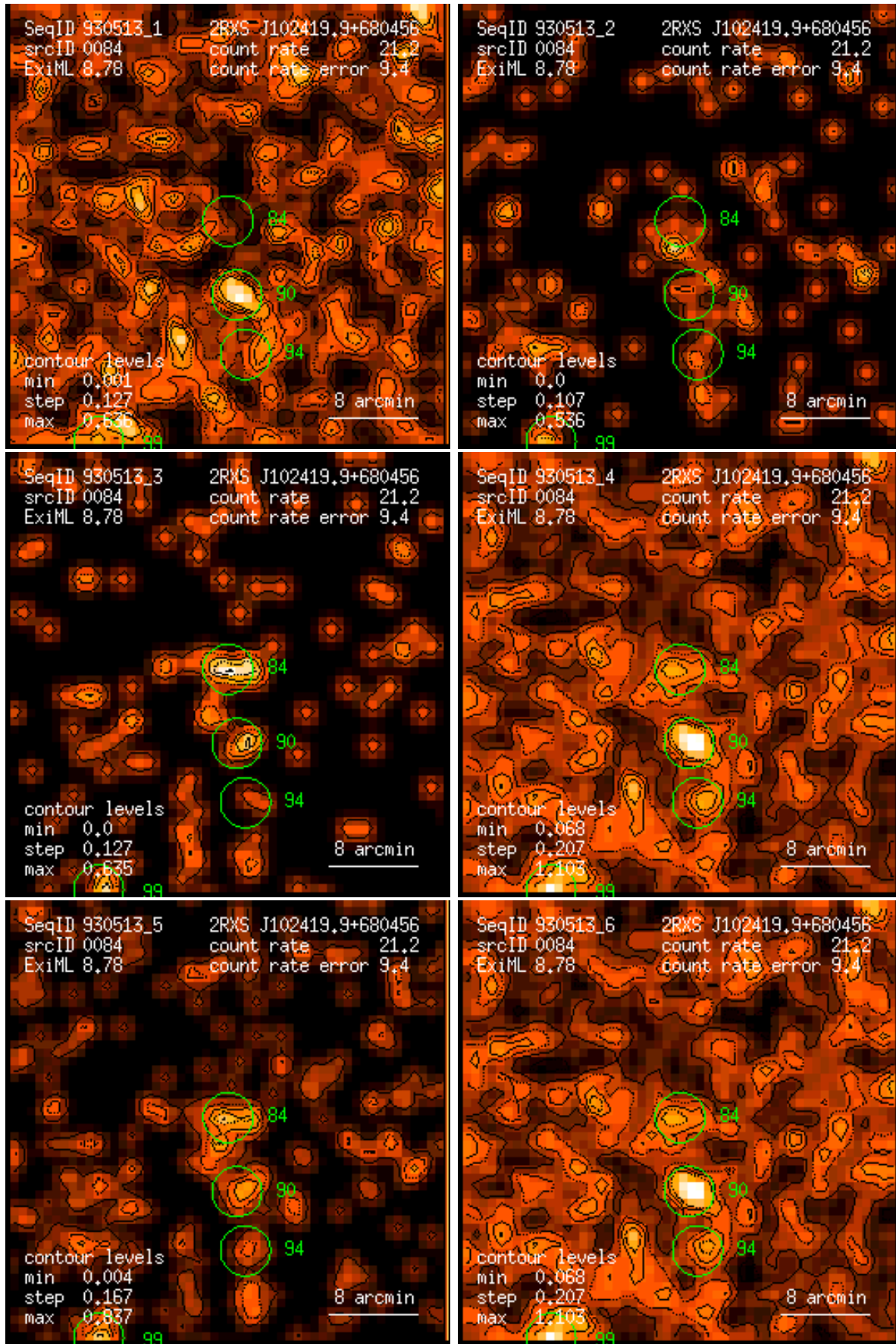
Figure 84: RASS 930513: detection 0084: band rate images, Gaussian filter: (1) PSPC channels 11 – 41, (2) 52 – 90, (3) 91 – 201, (4) 11 – 235, (5) 52 – 201, (6) 11 – 201. Broad band rates in counts/ks. Band rate contour levels in counts/ks/arcmin 2 .
