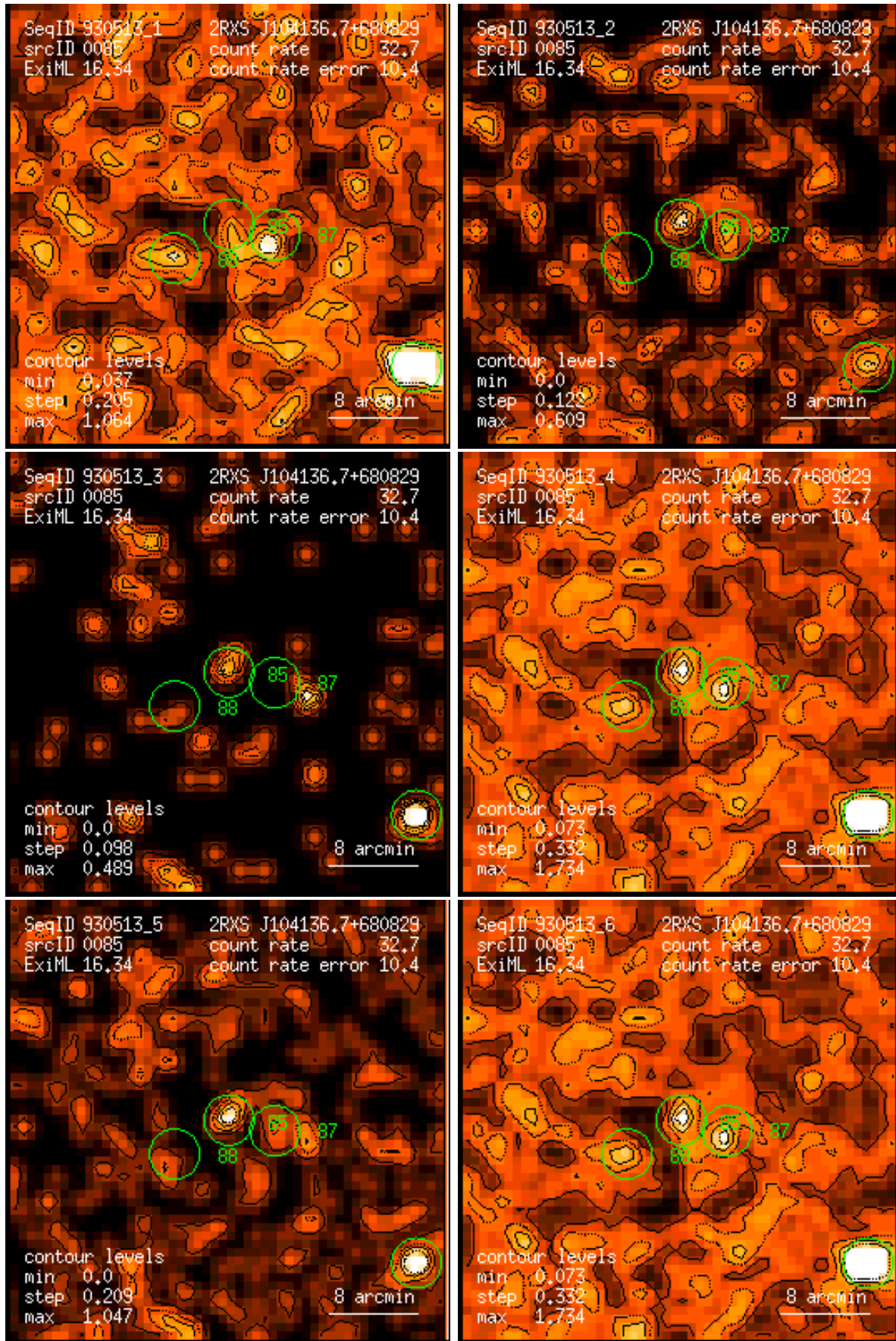
Figure 85: RASS 930513: detection 0085: band rate images, Gaussian filter: (1) PSPC channels 11 – 41, (2) 52 – 90, (3) 91 – 201, (4) 11 – 235, (5) 52 – 201, (6) 11 – 201. Broad band rates in counts/ks. Band rate contour levels in counts/ks/arcmin 2 .
