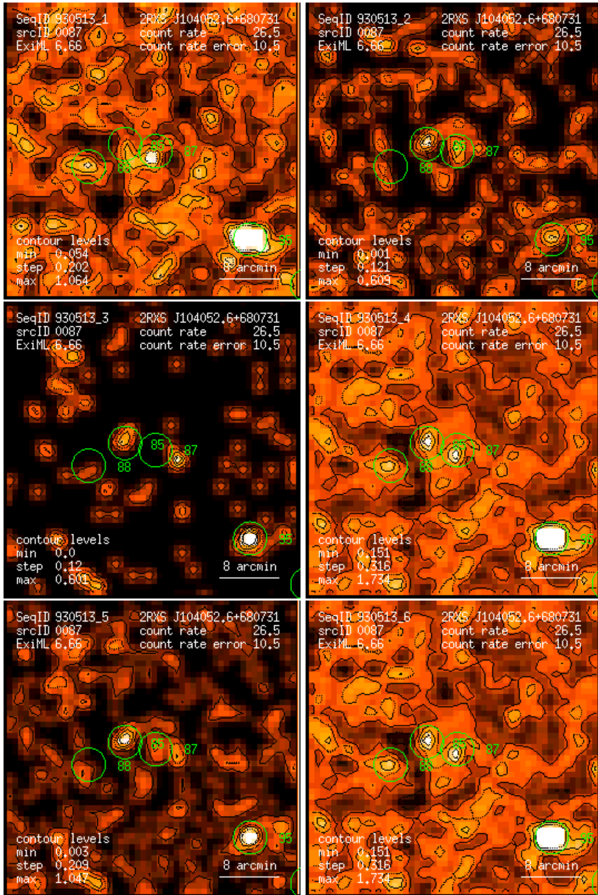
Figure 87: RASS 930513: detection 0087: band rate images, Gaussian filter: (1) PSPC channels 11 – 41, (2) 52 – 90, (3) 91 – 201, (4) 11 – 235, (5) 52 – 201, (6) 11 – 201. Broad band rates in counts/ks. Band rate contour levels in counts/ks/arcmin 2 .
