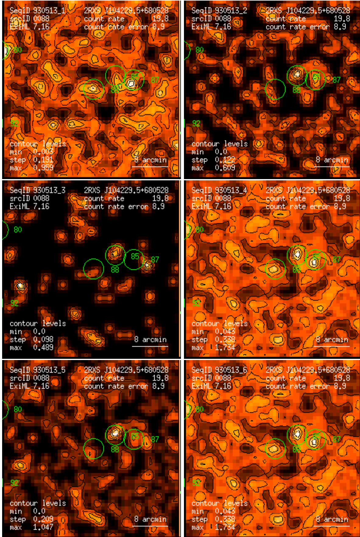
Figure 88: RASS 930513: detection 0088: band rate images, Gaussian filter: (1) PSPC channels 11 – 41, (2) 52 – 90, (3) 91 – 201, (4) 11 – 235, (5) 52 – 201, (6) 11 – 201. Broad band rates in counts/ks. Band rate contour levels in counts/ks/arcmin 2 .
