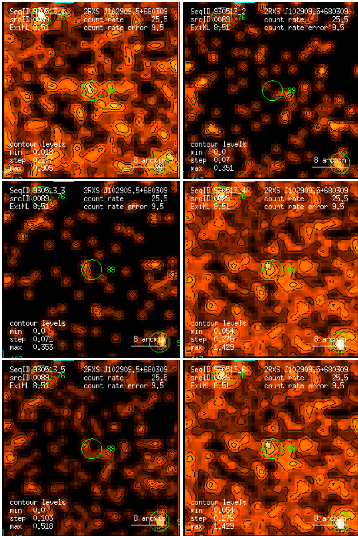
Figure 89: RASS 930513: detection 0089: band rate images, Gaussian filter: (1) PSPC channels 11 – 41, (2) 52 – 90, (3) 91 – 201, (4) 11 – 235, (5) 52 – 201, (6) 11 – 201. Broad band rates in counts/ks. Band rate contour levels in counts/ks/arcmin 2 .
