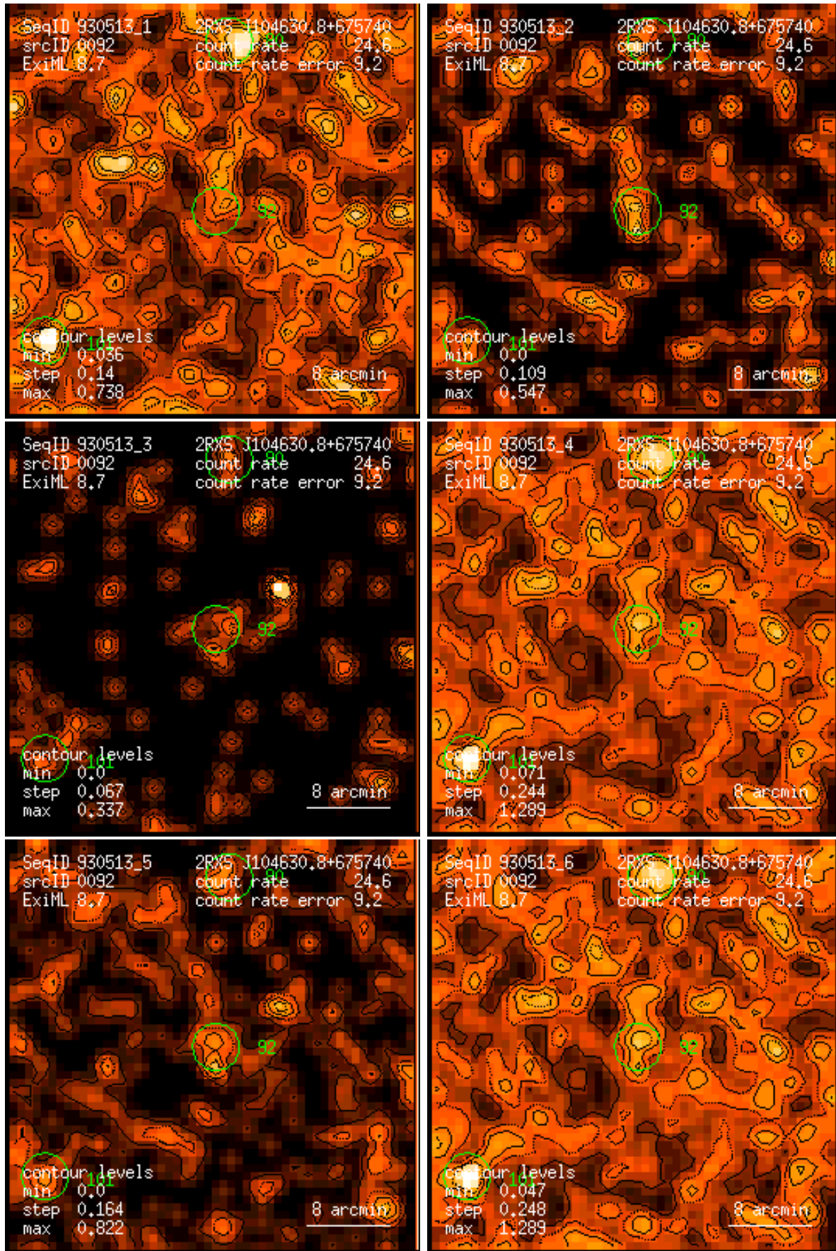
Figure 92: RASS 930513: detection 0092: band rate images, Gaussian filter: (1) PSPC channels 11 – 41, (2) 52 – 90, (3) 91 – 201, (4) 11 – 235, (5) 52 – 201, (6) 11 – 201. Broad band rates in counts/ks. Band rate contour levels in counts/ks/arcmin 2 .
