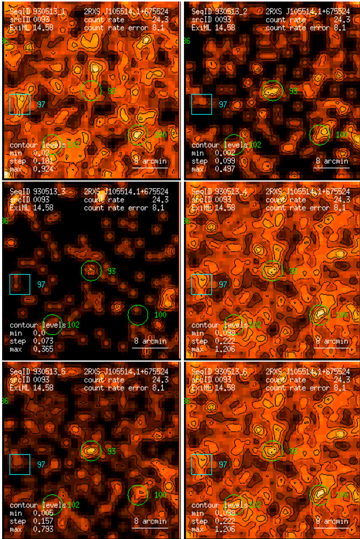
Figure 93: RASS 930513: detection 0093: band rate images, Gaussian filter: (1) PSPC channels 11 – 41, (2) 52 – 90, (3) 91 – 201, (4) 11 – 235, (5) 52 – 201, (6) 11 – 201. Broad band rates in counts/ks. Band rate contour levels in counts/ks/arcmin 2 .
