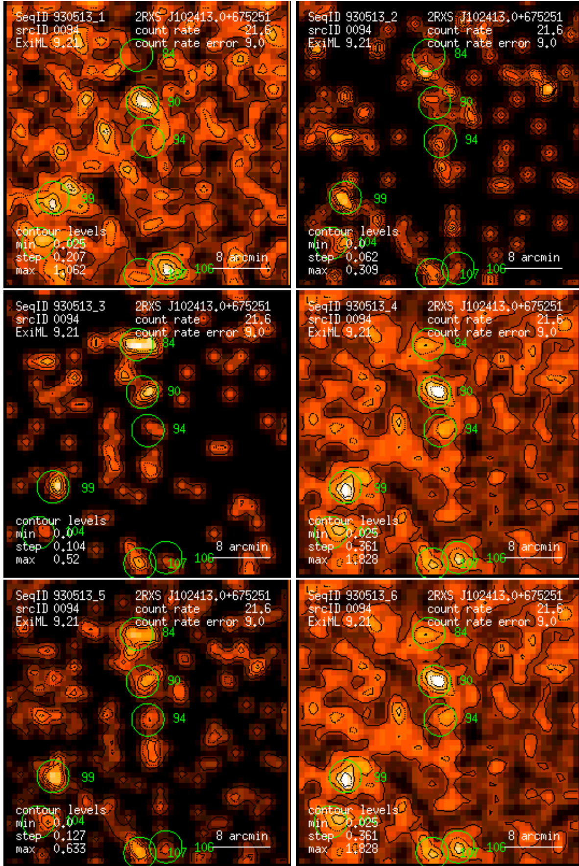
Figure 94: RASS 930513: detection 0094: band rate images, Gaussian filter: (1) PSPC channels 11 – 41, (2) 52 – 90, (3) 91 – 201, (4) 11 – 235, (5) 52 – 201, (6) 11 – 201. Broad band rates in counts/ks. Band rate contour levels in counts/ks/arcmin 2 .
