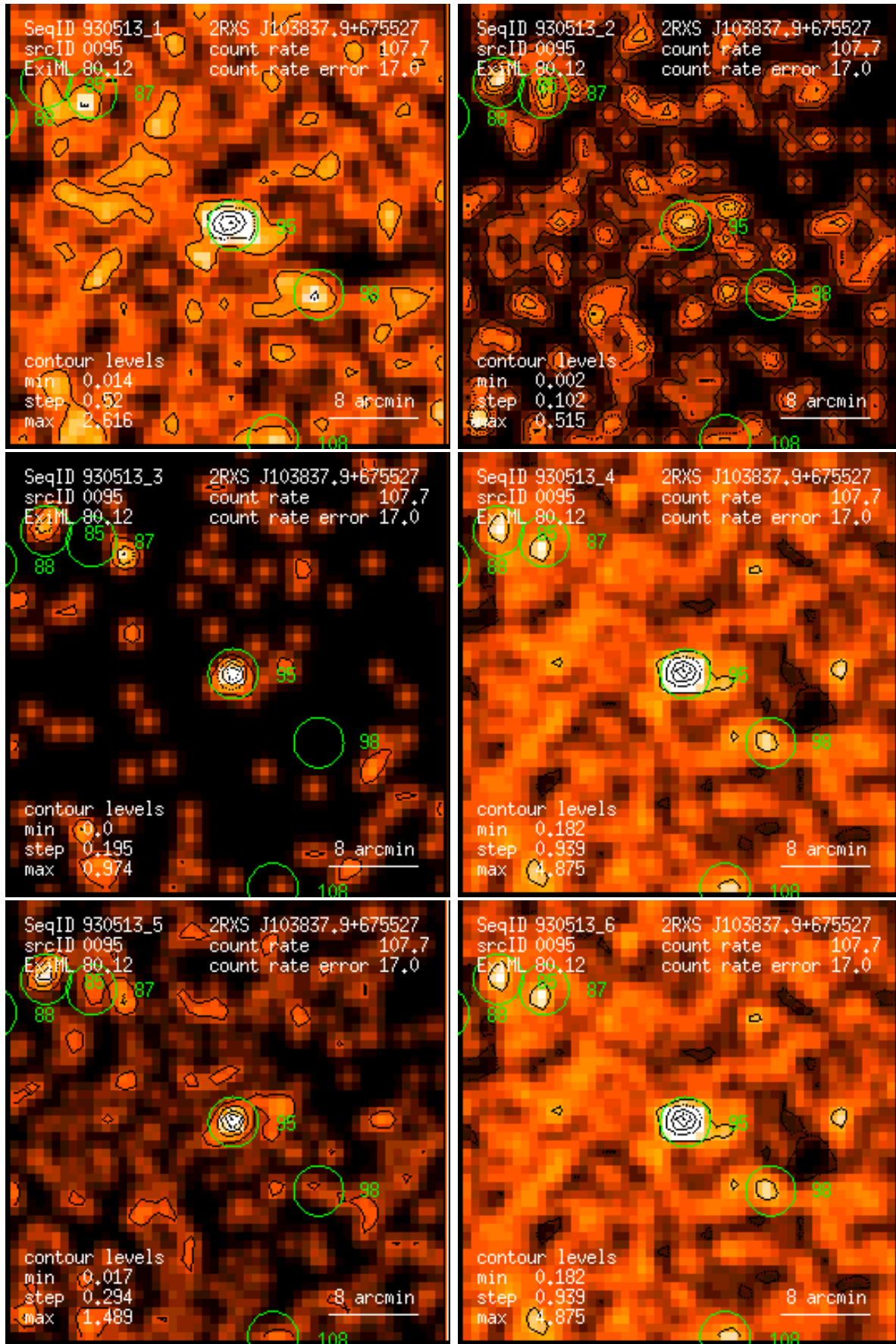
Figure 95: RASS 930513: detection 0095: band rate images, Gaussian filter: (1) PSPC channels 11 – 41, (2) 52 – 90, (3) 91 – 201, (4) 11 – 235, (5) 52 – 201, (6) 11 – 201. Broad band rates in counts/ks. Band rate contour levels in counts/ks/arcmin 2 .
