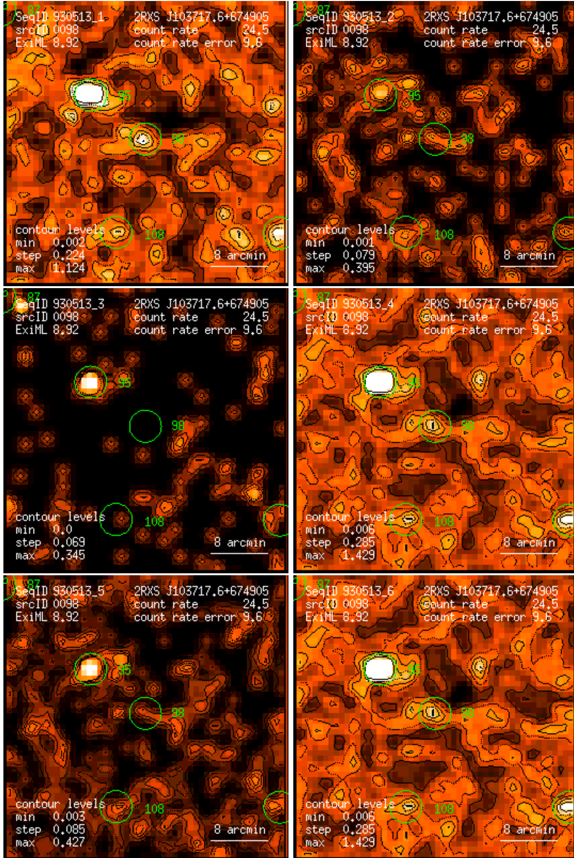
Figure 98: RASS 930513: detection 0098: band rate images, Gaussian filter: (1) PSPC channels 11 – 41, (2) 52 – 90, (3) 91 – 201, (4) 11 – 235, (5) 52 – 201, (6) 11 – 201. Broad band rates in counts/ks. Band rate contour levels in counts/ks/arcmin 2 .
