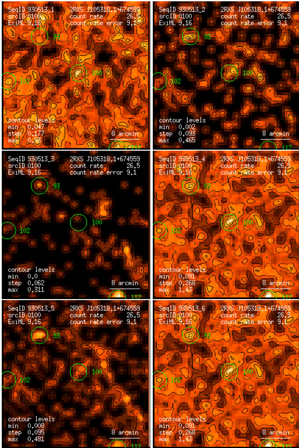
Figure 100: RASS 930513: detection 0100: band rate images, Gaussian filter: (1) PSPPC channels 11 – 41, (2) 52 – 90, (3) 91 – 201, (4) 11 – 235, (5) 52 – 201, (6) 11 – 201. Broad band rates in counts/ks. Band rate contour levels in counts/ks/arcmin 2 .
