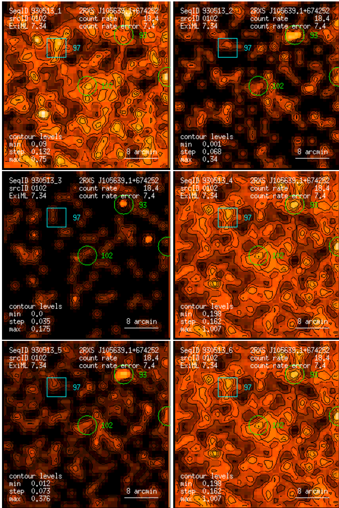
Figure 102: RASS 930513: detection 0102: band rate images, Gaussian filter: (1) PSPC channels 11 – 41, (2) 52 – 90, (3) 91 – 201, (4) 11 – 235, (5) 52 – 201, (6) 11 – 201. Broad band rates in counts/ks. Band rate contour levels in counts/ks/arcmin 2 .
