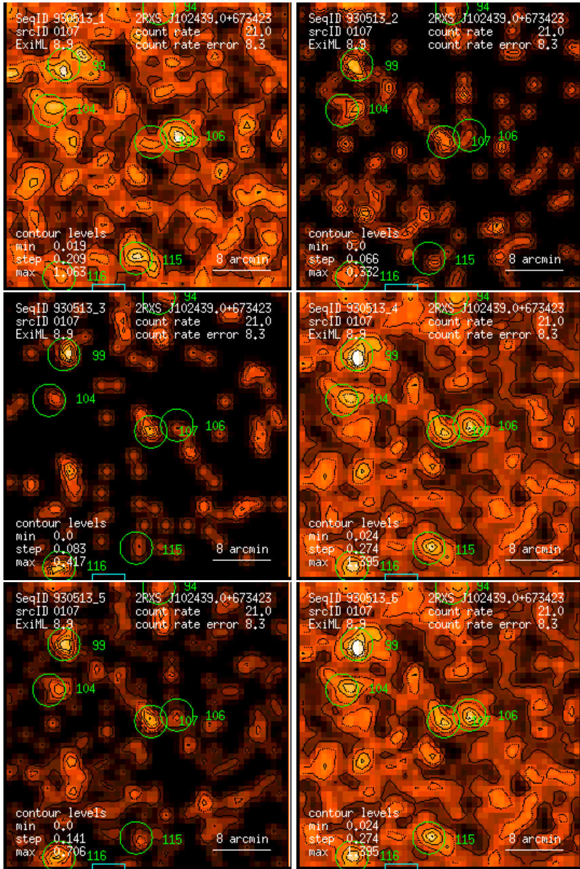
Figure 107: RASS 930513: detection 0107: band rate images, Gaussian filter: (1) PSPC channels 11 – 41, (2) 52 – 90, (3) 91 – 201, (4) 11 – 235, (5) 52 – 201, (6) 11 – 201. Broad band rates in counts/ks. Band rate contour levels in counts/ks/arcmin 2 .
