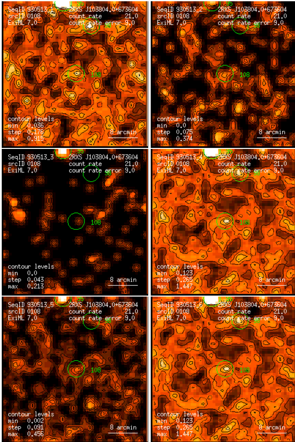
Figure 108: RASS 930513: detection 0108: band rate images, Gaussian filter: (1) PSPC channels 11 – 41, (2) 52 – 90, (3) 91 – 201, (4) 11 – 235, (5) 52 – 201, (6) 11 – 201. Broad band rates in counts/ks. Band rate contour levels in counts/ks/arcmin 2 .
