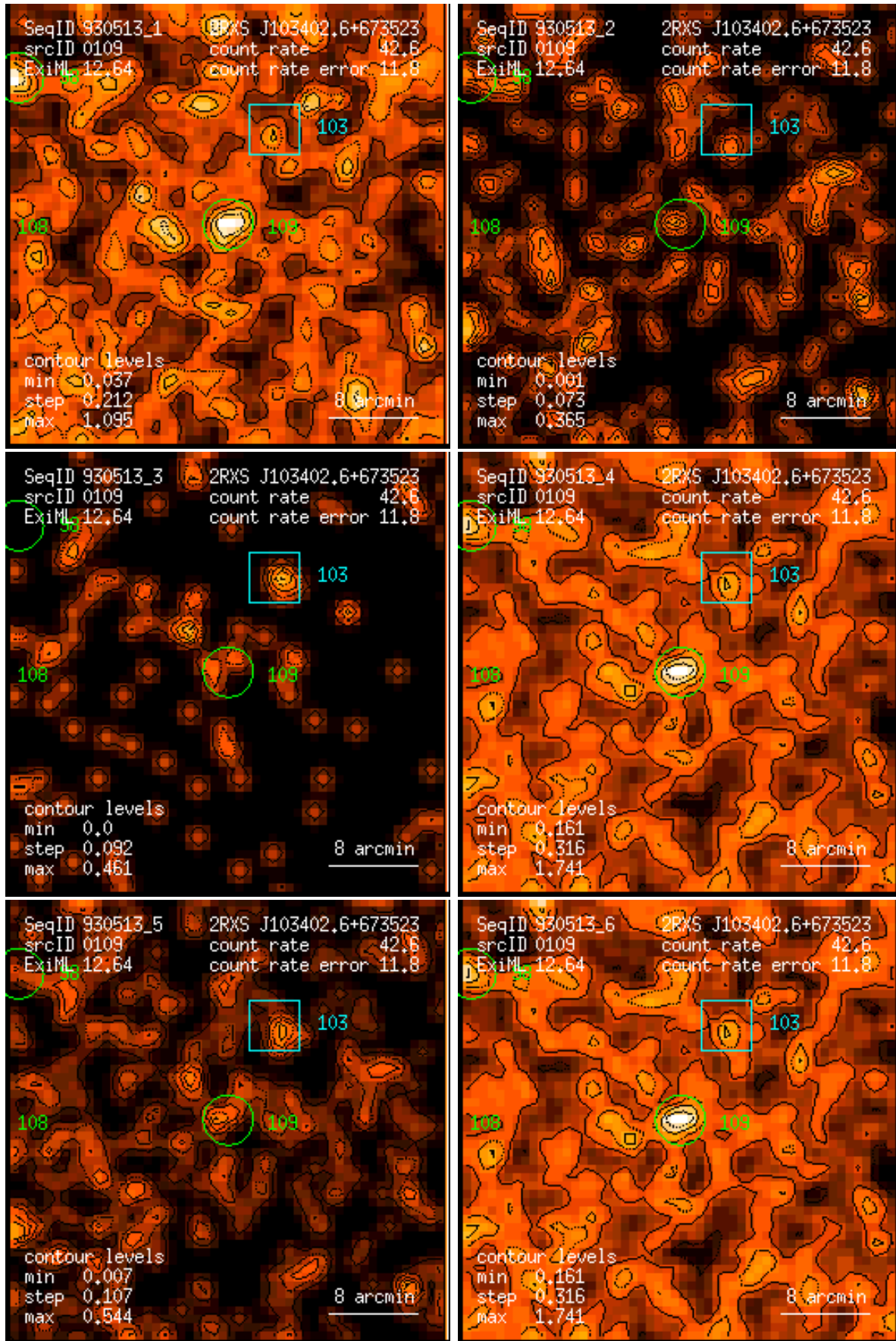
Figure 109: RASS 930513: detection 0109: band rate images, Gaussian filter: (1) PSPC channels 11 – 41, (2) 52 – 90, (3) 91 – 201, (4) 11 – 235, (5) 52 – 201, (6) 11 – 201. Broad band rates in counts/ks. Band rate contour levels in counts/ks/arcmin 2 .
