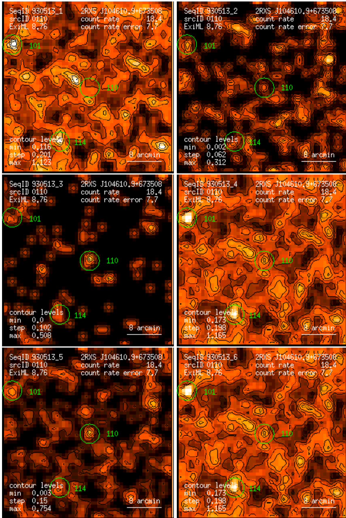
Figure 110: RASS 930513: detection 0110: band rate images, Gaussian filter: (1) PSPC channels 11 – 41, (2) 52 – 90, (3) 91 – 201, (4) 11 – 235, (5) 52 – 201, (6) 11 – 201. Broad band rates in counts/ks. Band rate contour levels in counts/ks/arcmin 2 .
