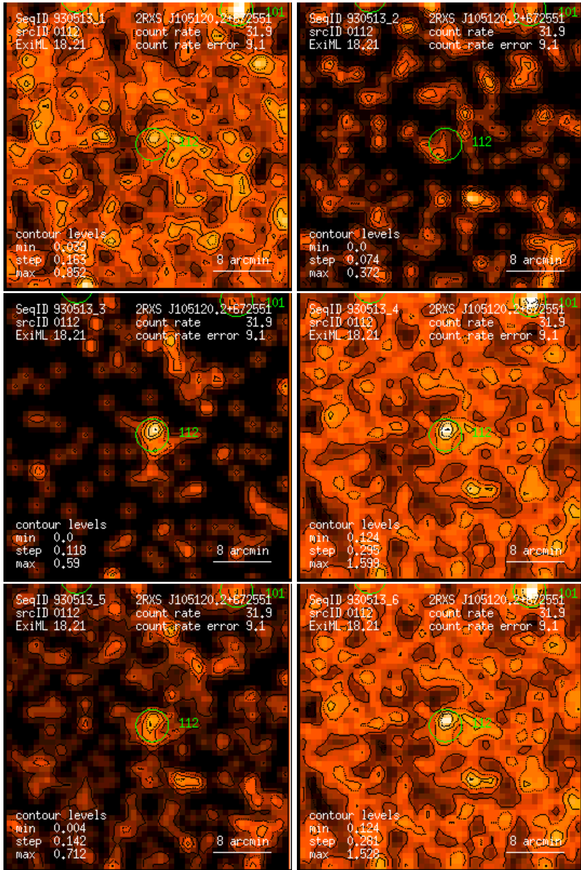
Figure 112: RASS 930513: detection 0112: band rate images, Gaussian filter: (1) PSPC channels 11 – 41, (2) 52 – 90, (3) 91 – 201, (4) 11 – 235, (5) 52 – 201, (6) 11 – 201. Broad band rates in counts/ks. Band rate contour levels in counts/ks/arcmin 2 .
