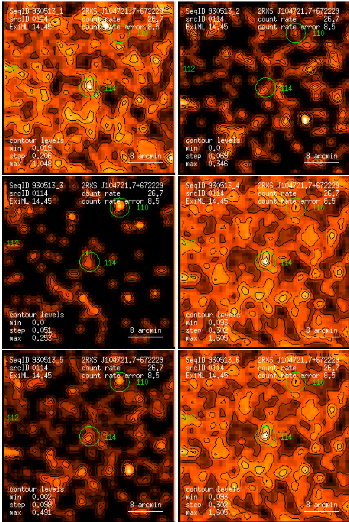
Figure 114: RASS 930513: detection 0114: band rate images, Gaussian filter: (1) PSPC channels 11 – 41, (2) 52 – 90, (3) 91 – 201, (4) 11 – 235, (5) 52 – 201, (6) 11 – 201. Broad band rates in counts/ks. Band rate contour levels in counts/ks/arcmin 2 .
