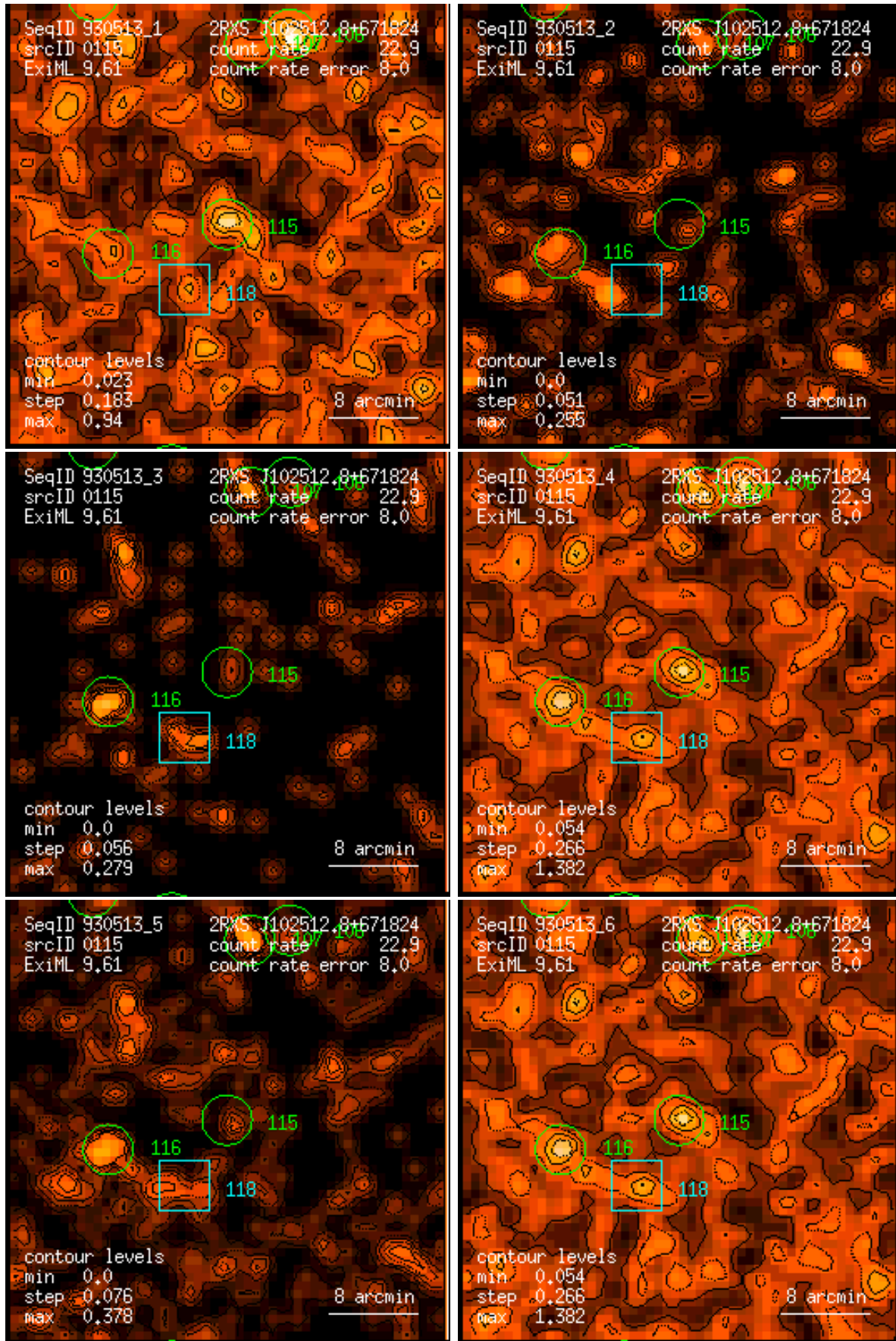
Figure 115: RASS 930513: detection 0115: band rate images, Gaussian filter: (1) PSPC channels 11 – 41, (2) 52 – 90, (3) 91 – 201, (4) 11 – 235, (5) 52 – 201, (6) 11 – 201. Broad band rates in counts/ks. Band rate contour levels in counts/ks/arcmin 2 .
