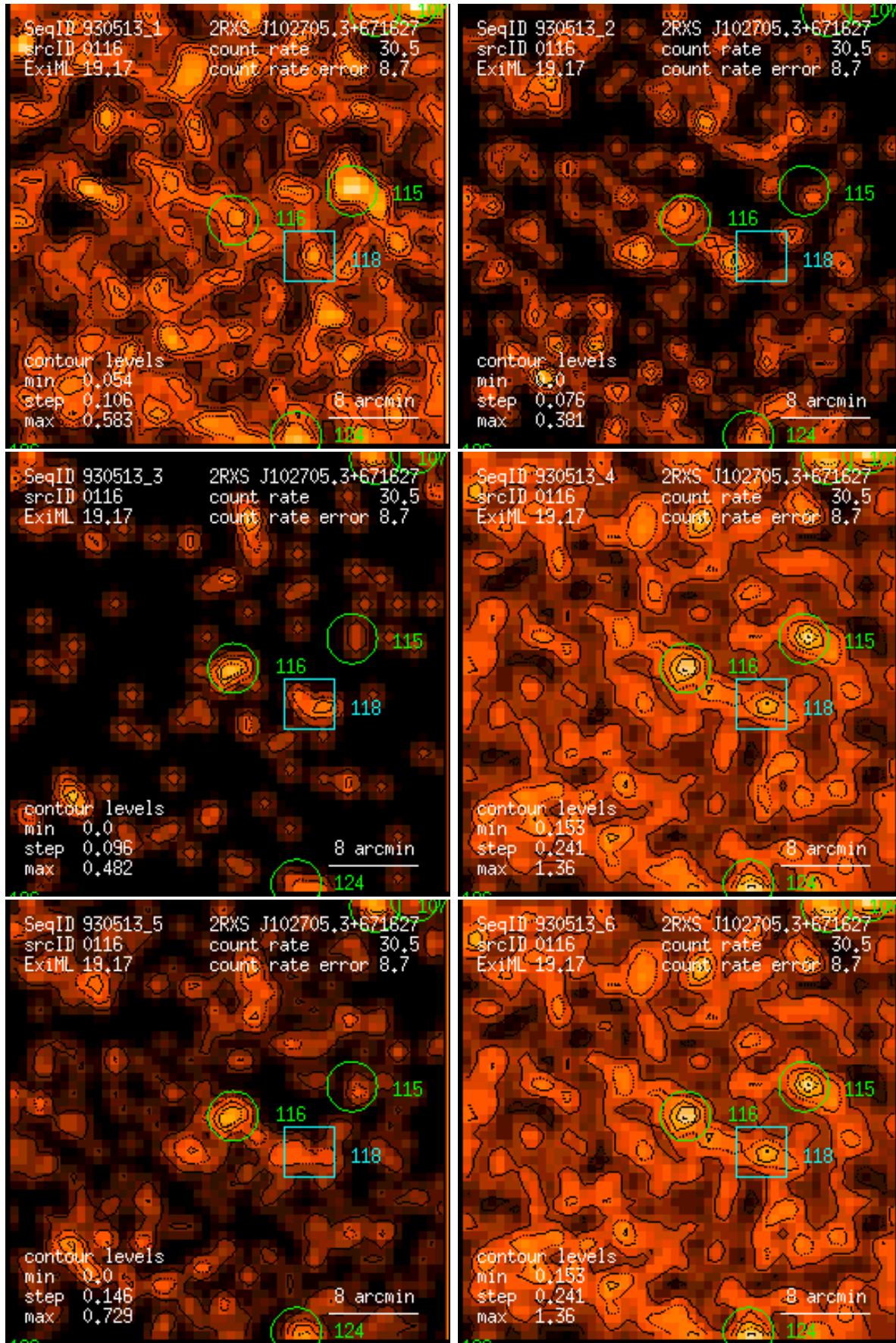
Figure 116: RASS 930513: detection 0116: band rate images, Gaussian filter: (1) PSPC channels 11 – 41, (2) 52 – 90, (3) 91 – 201, (4) 11 – 235, (5) 52 – 201, (6) 11 – 201. Broad band rates in counts/ks. Band rate contour levels in counts/ks/arcmin 2 .
