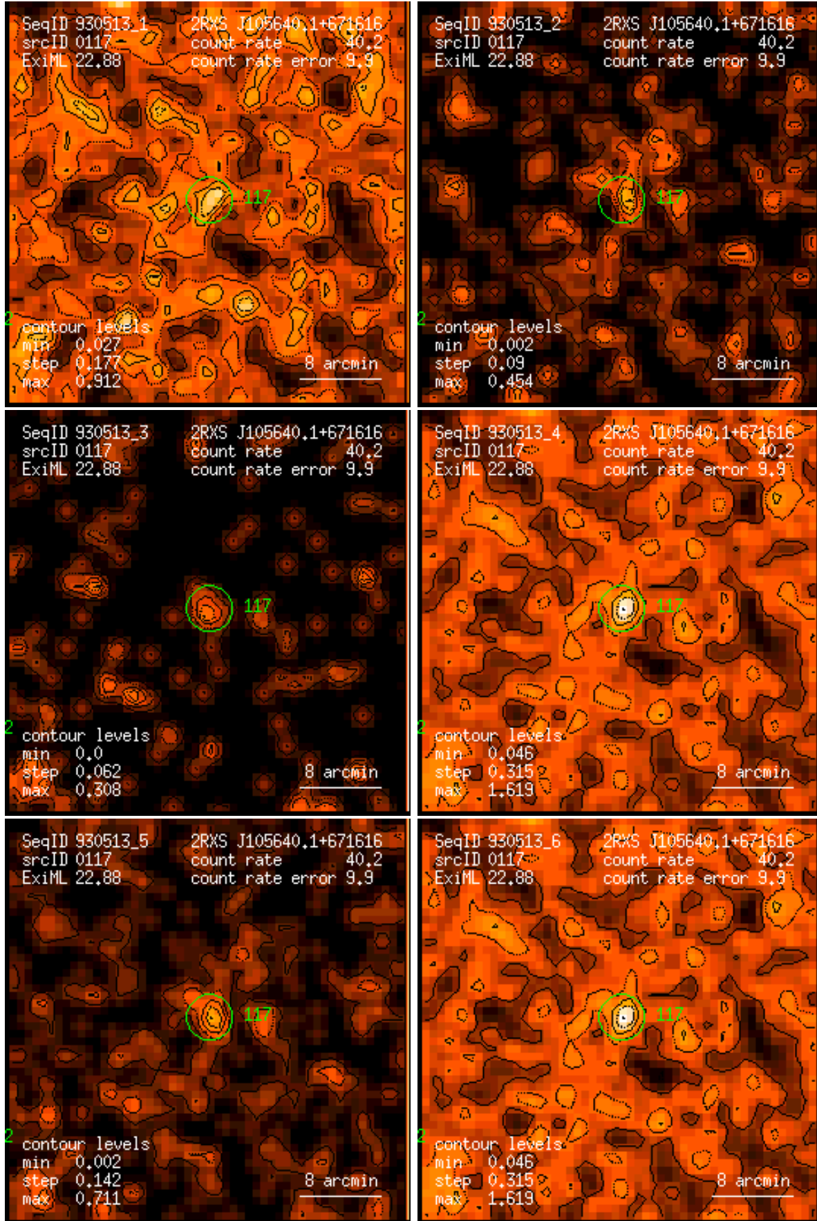
Figure 117: RASS 930513: detection 0117: band rate images, Gaussian filter: (1) PSPC channels 11 – 41, (2) 52 – 90, (3) 91 – 201, (4) 11 – 235, (5) 52 – 201, (6) 11 – 201. Broad band rates in counts/ks. Band rate contour levels in counts/ks/arcmin 2 .
