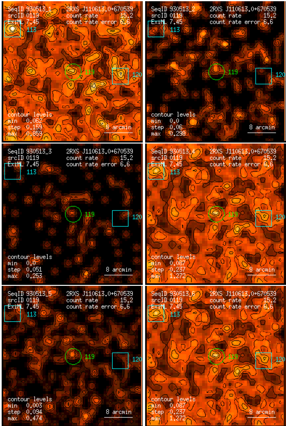
Figure 119: RASS 930513: detection 0119: band rate images, Gaussian filter: (1) PSPC channels 11 – 41, (2) 52 – 90, (3) 91 – 201, (4) 11 – 235, (5) 52 – 201, (6) 11 – 201. Broad band rates in counts/ks. Band rate contour levels in counts/ks/arcmin 2 .
