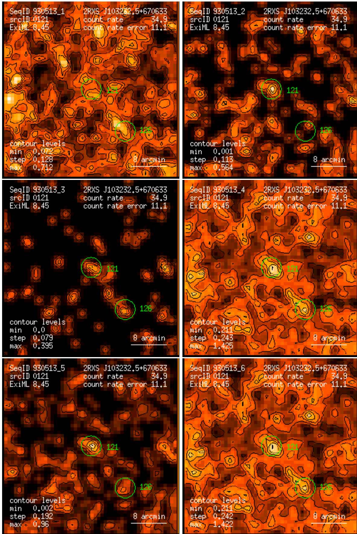
Figure 121: RASS 930513: detection 0121: band rate images, Gaussian filter: (1) PSPC channels 11 – 41, (2) 52 – 90, (3) 91 – 201, (4) 11 – 235, (5) 52 – 201, (6) 11 – 201. Broad band rates in counts/ks. Band rate contour levels in counts/ks/arcmin 2 .
