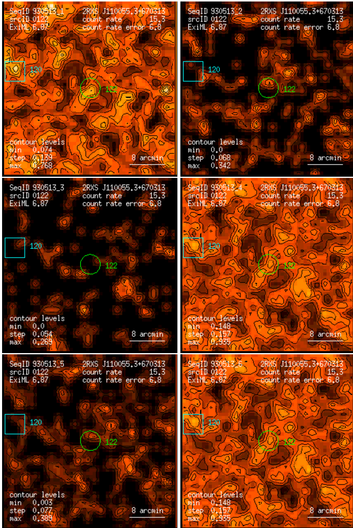
Figure 122: RASS 930513: detection 0122: band rate images, Gaussian filter: (1) PSPC channels 11 – 41, (2) 52 – 90, (3) 91 – 201, (4) 11 – 235, (5) 52 – 201, (6) 11 – 201. Broad band rates in counts/ks. Band rate contour levels in counts/ks/arcmin 2 .
