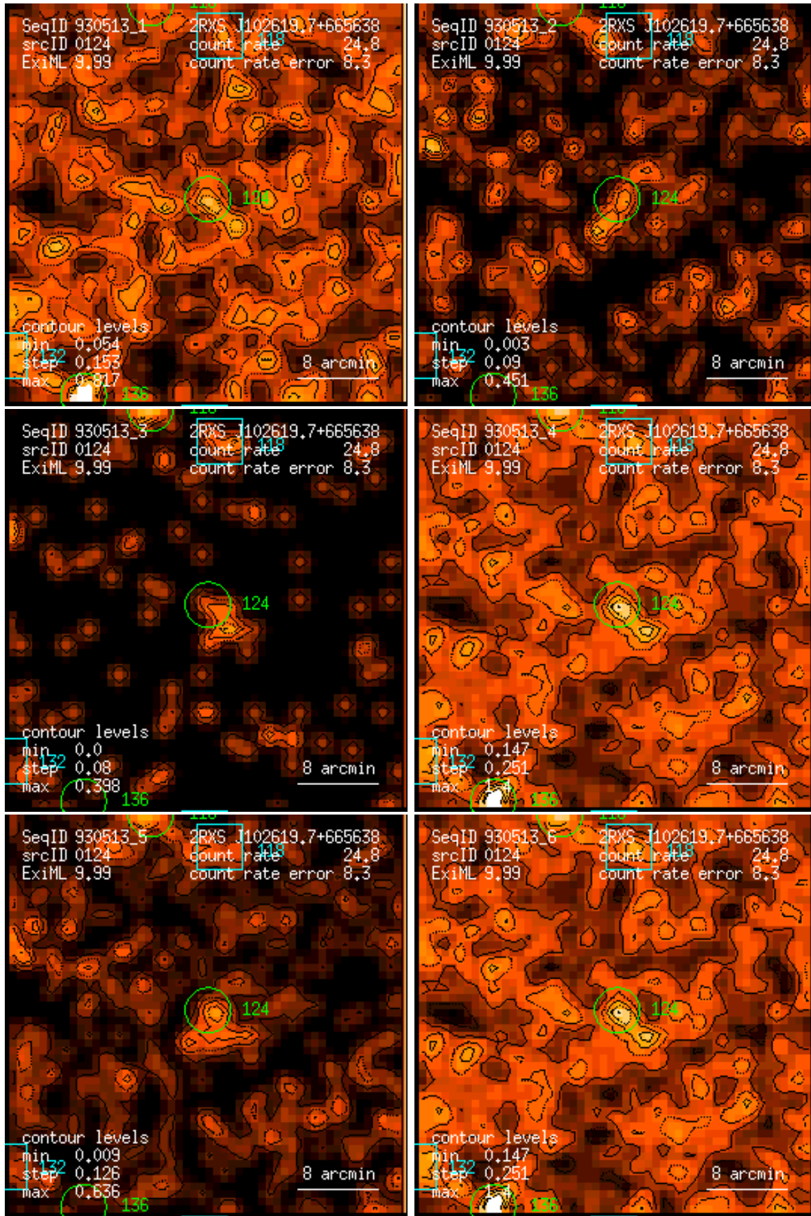
Figure 124: RASS 930513: detection 0124: band rate images, Gaussian filter: (1) PSPC channels 11 – 41, (2) 52 – 90, (3) 91 – 201, (4) 11 – 235, (5) 52 – 201, (6) 11 – 201. Broad band rates in counts/ks. Band rate contour levels in counts/ks/arcmin 2 .
