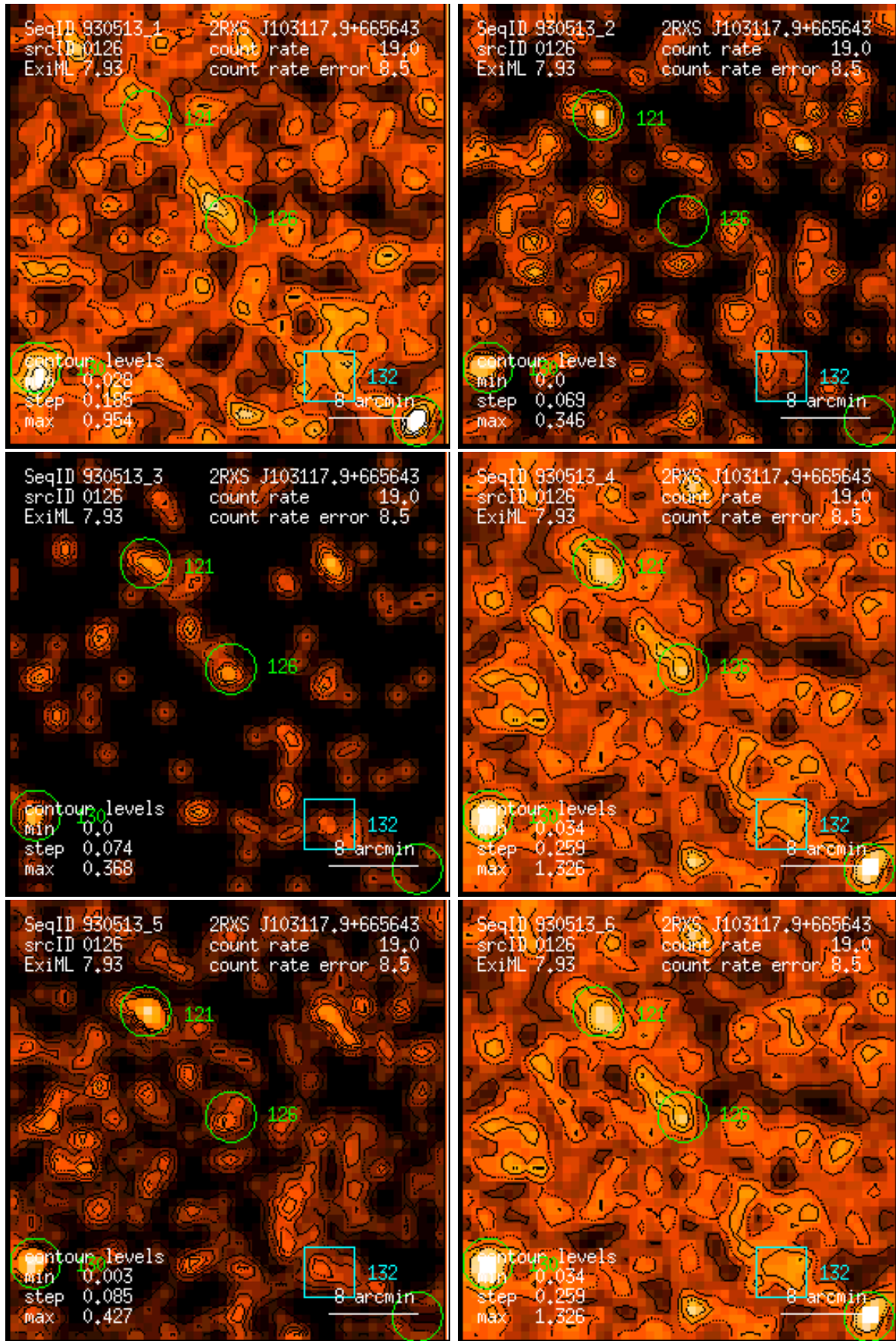
Figure 126: RASS 930513: detection 0126: band rate images, Gaussian filter: (1) PSPC channels 11 – 41, (2) 52 – 90, (3) 91 – 201, (4) 11 – 235, (5) 52 – 201, (6) 11 – 201. Broad band rates in counts/ks. Band rate contour levels in counts/ks/arcmin 2 .
