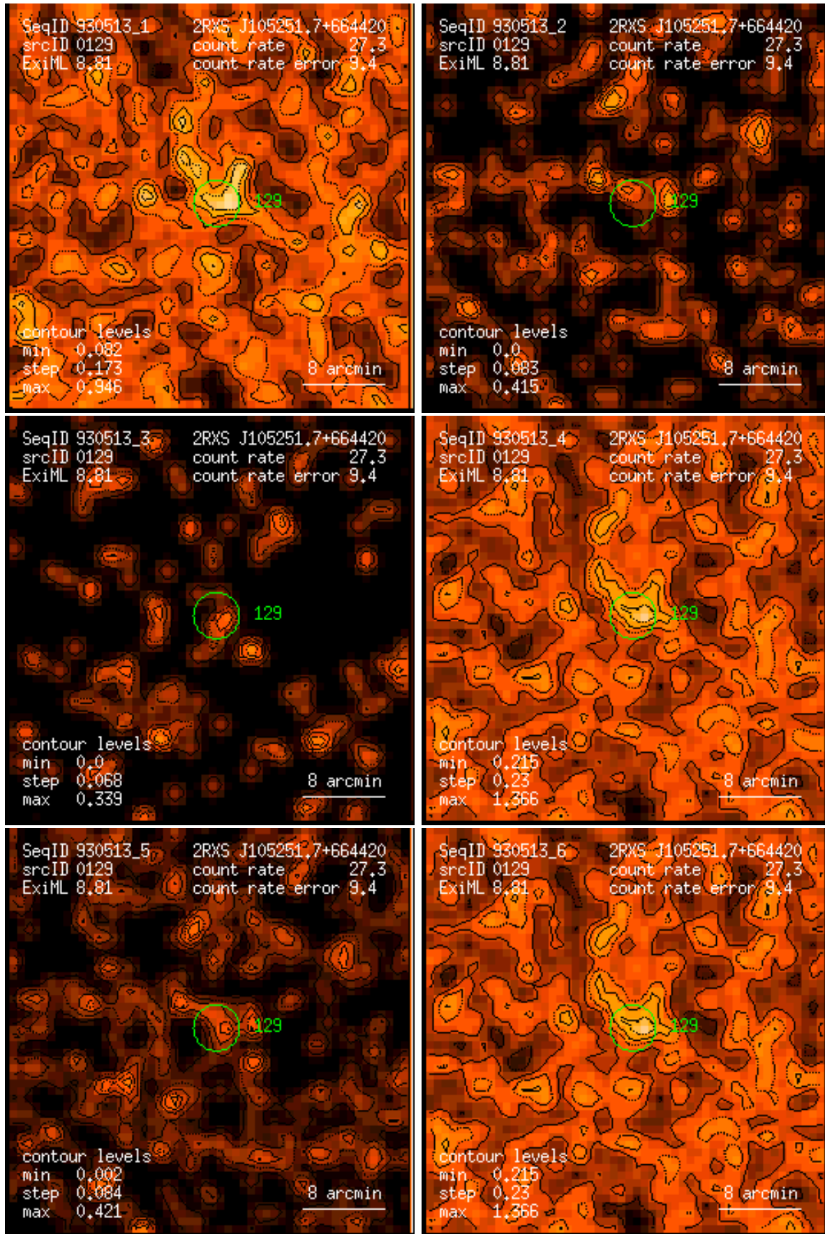
Figure 129: RASS 930513: detection 0129: band rate images, Gaussian filter: (1) PSPC channels 11 – 41, (2) 52 – 90, (3) 91 – 201, (4) 11 – 235, (5) 52 – 201, (6) 11 – 201. Broad band rates in counts/ks. Band rate contour levels in counts/ks/arcmin 2 .
