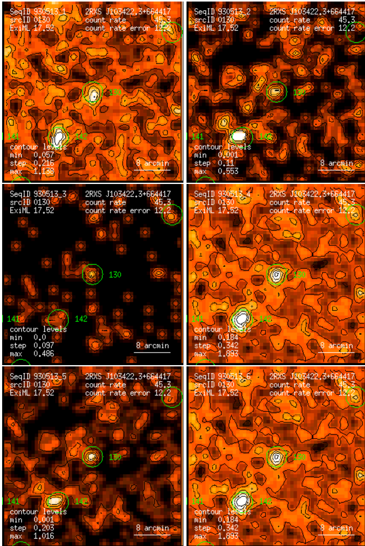
Figure 130: RASS 930513: detection 0130: band rate images, Gaussian filter: (1) PSPC channels 11 – 41, (2) 52 – 90, (3) 91 – 201, (4) 11 – 235, (5) 52 – 201, (6) 11 – 201. Broad band rates in counts/ks. Band rate contour levels in counts/ks/arcmin 2 .
