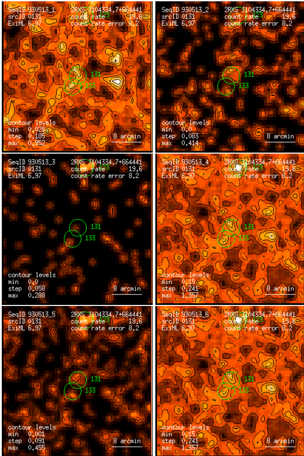
Figure 131: RASS 930513: detection 0131: band rate images, Gaussian filter: (1) PSPC channels 11 – 41, (2) 52 – 90, (3) 91 – 201, (4) 11 – 235, (5) 52 – 201, (6) 11 – 201. Broad band rates in counts/ks. Band rate contour levels in counts/ks/arcmin 2 .
