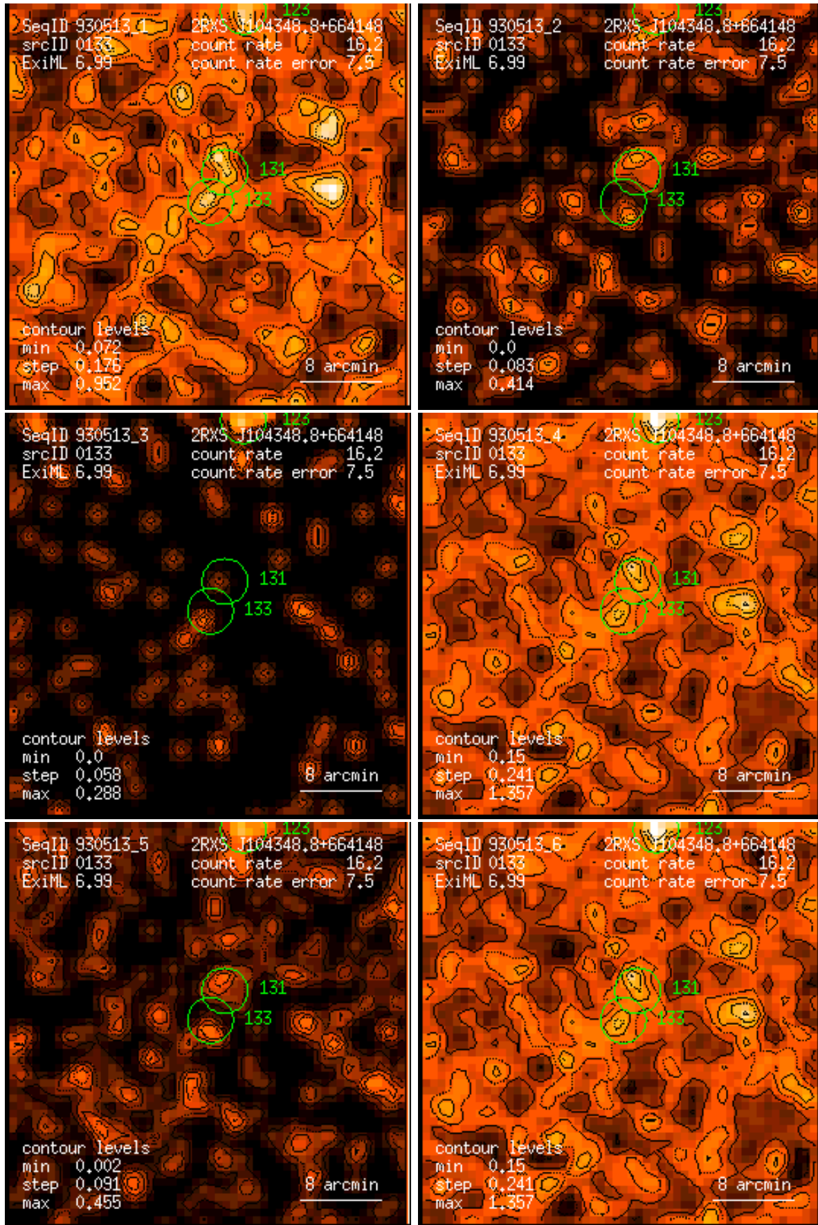
Figure 133: RASS 930513: detection 0133: band rate images, Gaussian filter: (1) PSPC channels 11 – 41, (2) 52 – 90, (3) 91 – 201, (4) 11 – 235, (5) 52 – 201, (6) 11 – 201. Broad band rates in counts/ks. Band rate contour levels in counts/ks/arcmin 2 .
