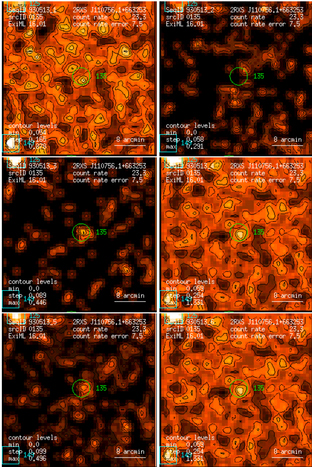
Figure 135: RASS 930513: detection 0135: band rate images, Gaussian filter: (1) PSPC channels 11 – 41, (2) 52 – 90, (3) 91 – 201, (4) 11 – 235, (5) 52 – 201, (6) 11 – 201. Broad band rates in counts/ks. Band rate contour levels in counts/ks/arcmin 2 .
