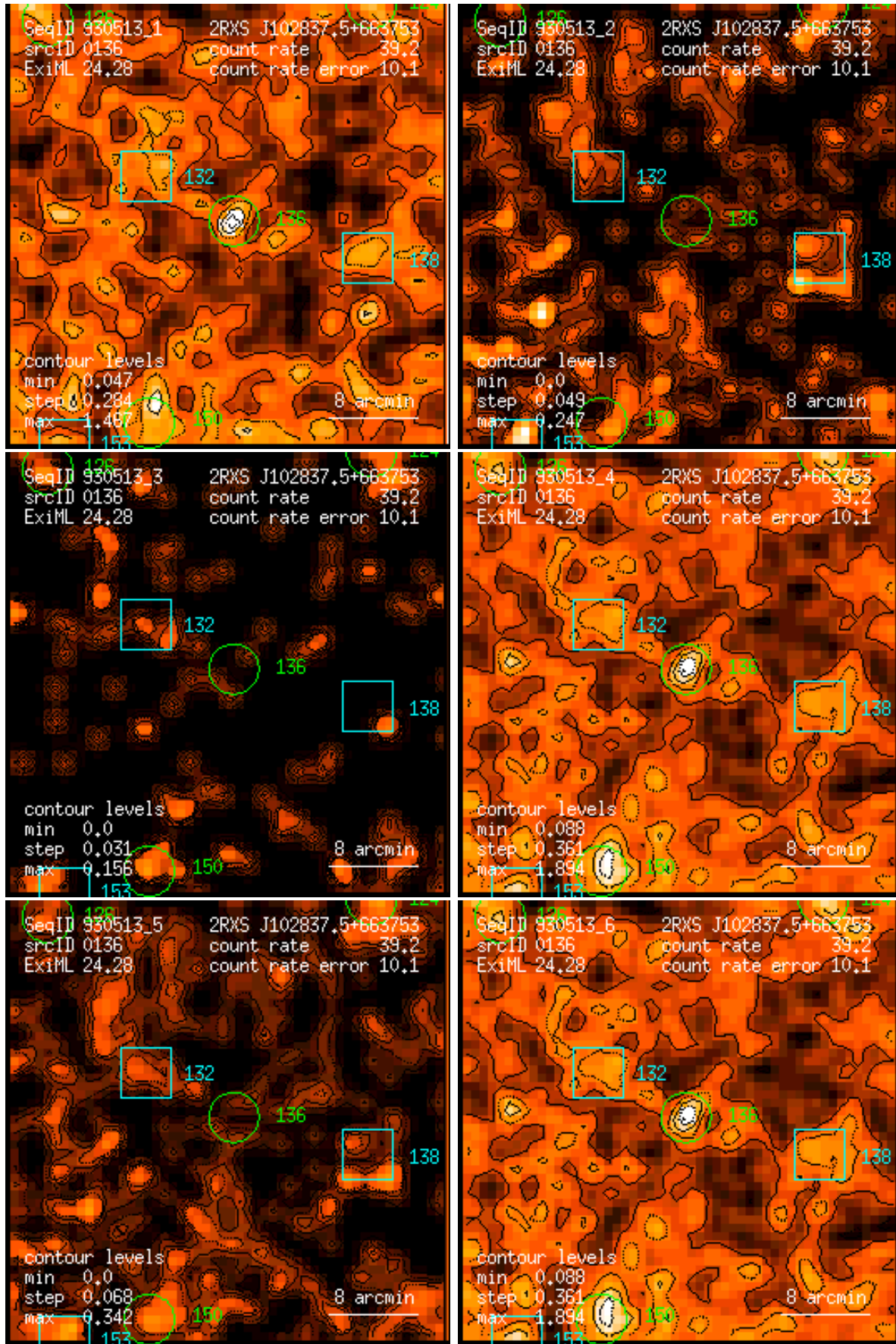
Figure 136: RASS 930513: detection 0136: band rate images, Gaussian filter: (1) PSPC channels 11 – 41, (2) 52 – 90, (3) 91 – 201, (4) 11 – 235, (5) 52 – 201, (6) 11 – 201. Broad band rates in counts/ks. Band rate contour levels in counts/ks/arcmin 2 .
