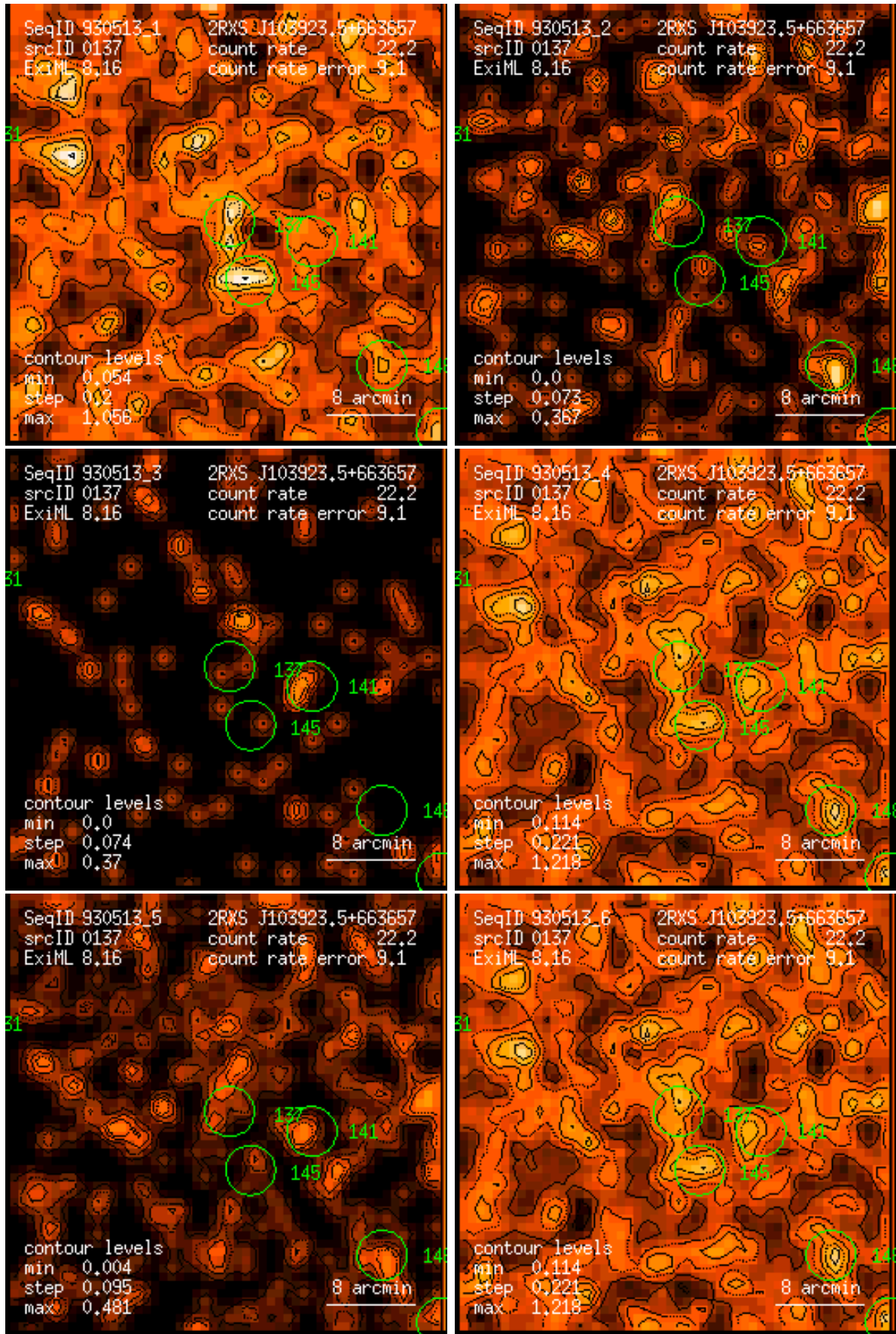
Figure 137: RASS 930513: detection 0137: band rate images, Gaussian filter: (1) PSPC channels 11 – 41, (2) 52 – 90, (3) 91 – 201, (4) 11 – 235, (5) 52 – 201, (6) 11 – 201. Broad band rates in counts/ks. Band rate contour levels in counts/ks/arcmin 2 .
